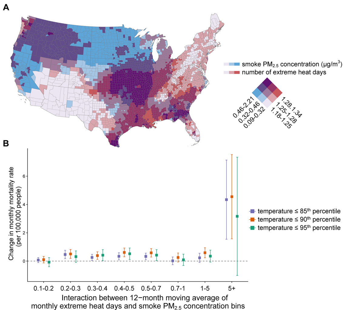
10 11 Fig. 4. Interaction effects between extreme heat and smoke PM_{2.5} on all-cause 12 mortality rate. A: This bivariate choropleth map shows the spatial distribution of 12- 13 month moving average of smoke PM_{2.5} concentrations and 12-month moving average 14 number of extreme heat days in each county, 2007-2020. Darker blue indicates higher 15 average smoke PM_{2.5} concentrations; darker red indicates more average extreme heat 16 days; and darker purple indicates higher values of both variables. B: The interaction 17 effects between 12-month moving average number of extreme heat days (a continuous 18 variable) and 12-month moving average of smoke PM_{2.5} concentration bins (a categorial 19 variable). The error bars indicate 95% confidence intervals. Extreme heat days were 20 defined as days with daily mean air temperature higher than the county's 90 th (main 21 analysis), 85 th , or 95 th (sensitivity analyses) percentile warm season air temperature 22 (May to September, 2007-2020).
