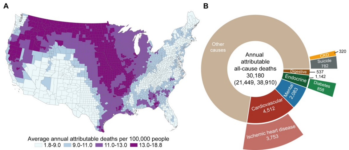
4 Fig. 3. Average annual mortality burden attributable to long-term smoke PM 2.5 5 exposure. A: The spatial distribution of average annual all-cause deaths (per 100,000 6 people) attributable to long-term smoke PM 2.5 exposure (12-month moving average). B: 7 Estimated average annual all-cause and cause-specific deaths attributable to long-term 8 smoke PM 2.5 exposure.
