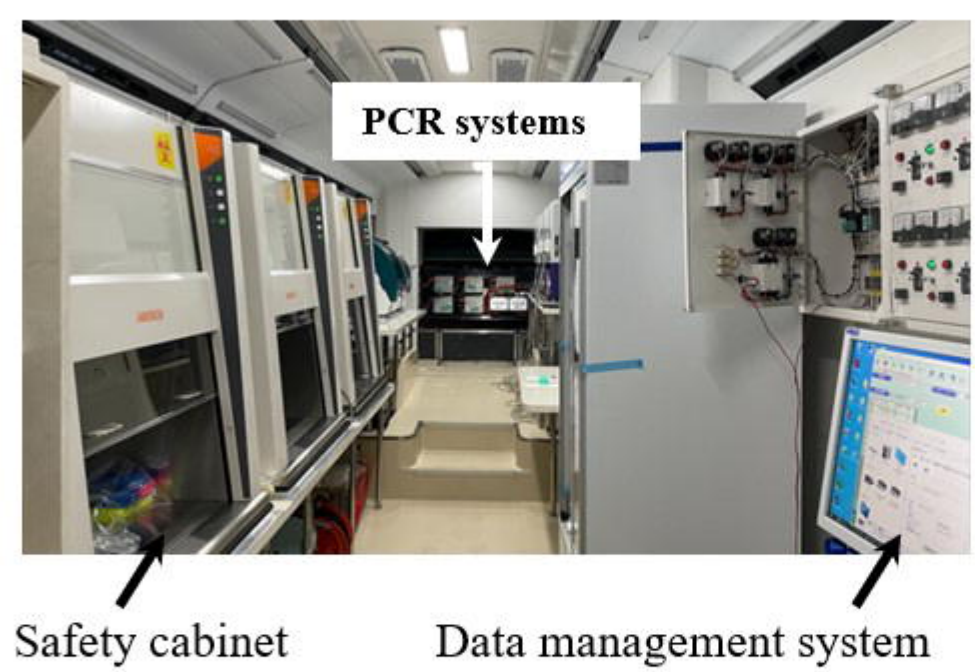
Interior of mobile laboratory (Motorcoach-type)
