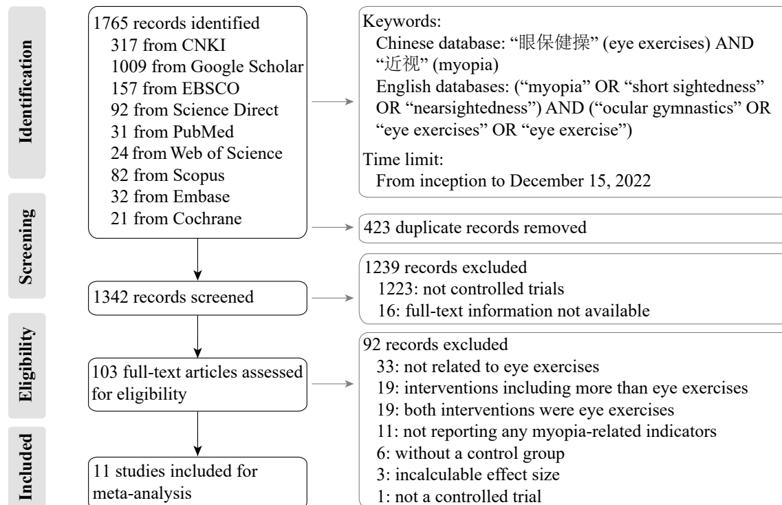
Figure 1: Study selection
