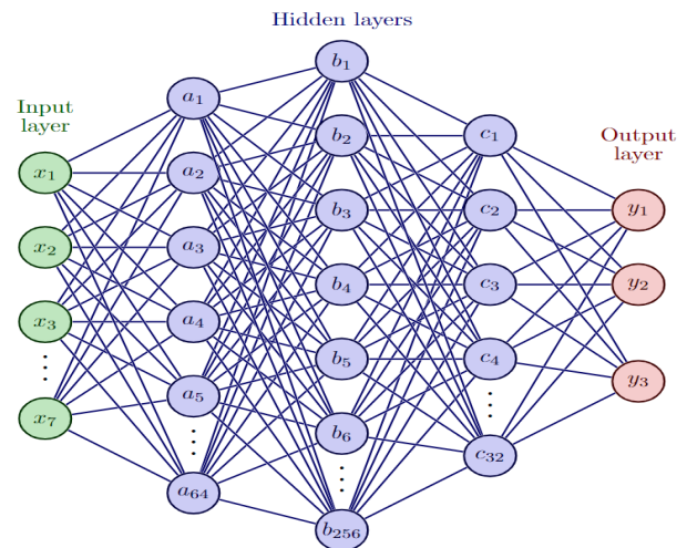
Figure 4. Architecture of Clinical Factors Neural Network
