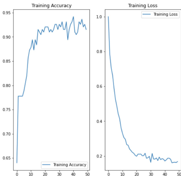
Figure 5. Accuracy of the CFNN in classifying the training data across 50 epochs (left) and value of categorical cross-entropy loss function for each epoch (right).
