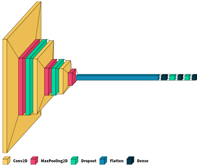
Figure 2. Visualization of the CNN's Architecture
