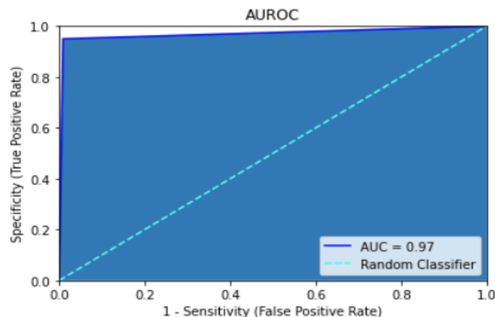
Figure 7. Visualization of the CNN's AUROC versus a random classifier (dashed lines). AUROCs closer to 1 indicate a greater ability to seperater the 3 different classes.
