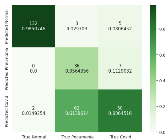
Figure 8. Confusion matrix comparing the true labels for 297 CT scans and the predicted labels by 3 independent radiologists. The radiologists' accuracy was 73.4%.
