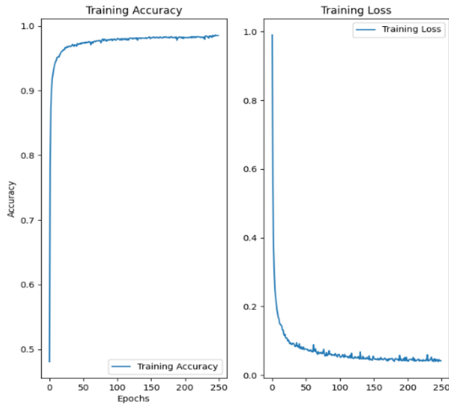
Figure 3. Accuracy of the CNN in classifying the training data across 250 epochs (left) and value of categorical cross-entropy loss function for each epoch (right).
