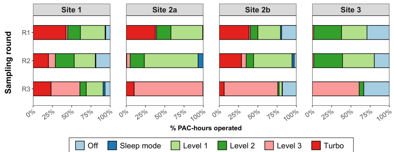
Fig. 1. The measured % time of PACs operated under different fan speed levels. R1: round 1; R2: round 2; R3: round 3. The PACs were initially set to operate on Auto-mode during round 1 and round 2, and fan speed level 3 during round 3.
