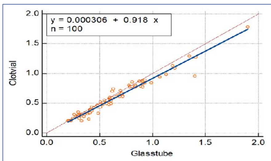
Fig 2: Deming regression showing the error measured during the analysis of values obtained from clot activator vacutainer and glass vial collection tube
