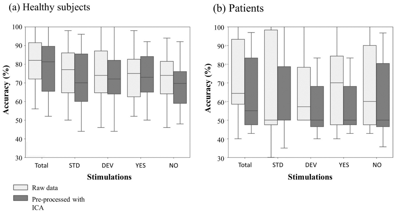
Figure 3: Offline classification results with and without ICA correction
