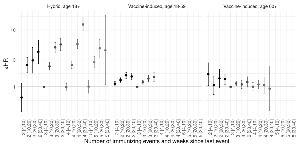
Figure 3. Adjusted hazard ratio (HR) of infection with Omicron SARS-CoV-2 by number of immunizing events. 4 to 10 weeks after the third immunizing event was the reference group. Error bars depict 95% confidence intervals. Underlying numbers can be found in Table S5.
