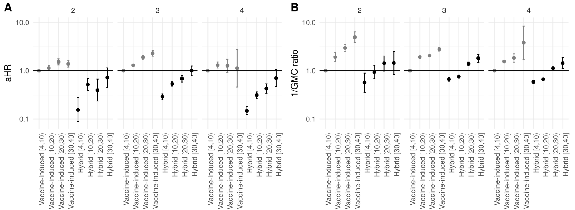
Figure 1. A. Adjusted hazard ratio (aHR) of infection with Omicron SARS-CoV-2 by hybrid or vaccine-induced immunity, stratified by the number of prior immunizing events. B. One divided by the adjusted geometric mean concentration (GMC) ratio of S-antibodies. In both analyses, 4 to 10 weeks after the last vaccination for vaccine-only immunity was the reference group. The group with 4 immunizing events only includes participants aged 60 and older, because younger people were not eligible for 4 vaccinations. Error bars depict 95% confidence intervals.
