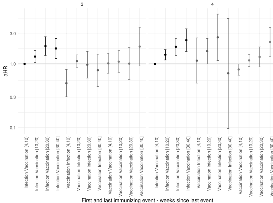
Figure 2. Adjusted hazard ratio (aHR) of infection with Omicron SARS-CoV-2 by the type of first and last immunizing event, stratified by the number of exposures. 4 to 10 weeks after the last vaccination for infection first and vaccination last was the reference. Error bars depict 95% confidence intervals. Underlying numbers can be found in Table S4.
