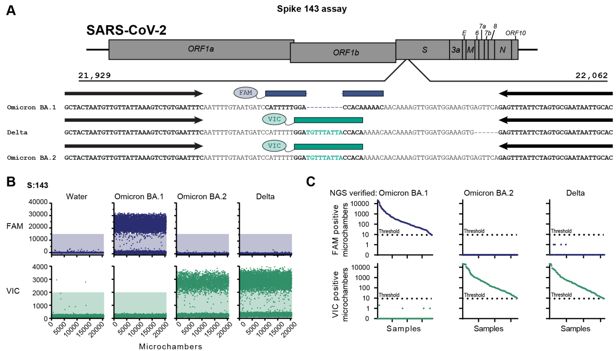
236 237 Fig 2: Digital PCR assay for the determination of the Omicron BA.1, and Delta or Omicron BA.2 238 lineages. (A) Schematic showing annealing locations of primers (black arrows) and probes 239 (colored boxes) on the SARS-CoV-2 genome. (B) Representative fluorescence intensities of dPCR 240 microchambers for synthetic DNA constructs. Positive microchambers are those exceeding
