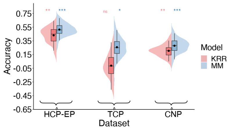
Supplementary Figure 6 - Model performance after regressing out age, sex and head motion (mean FD)
