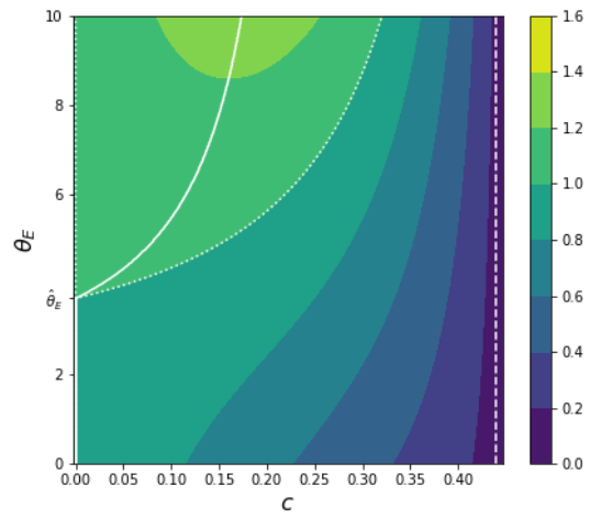
(b) Relative escape pressure \hat{P}_a(c) .
