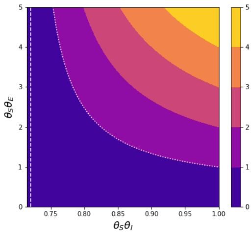
(a) Relative escape pressure \hat{P}_a(1) .
