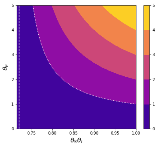
(c) Relative escape pressure \hat{P}_{a'}(1) .
