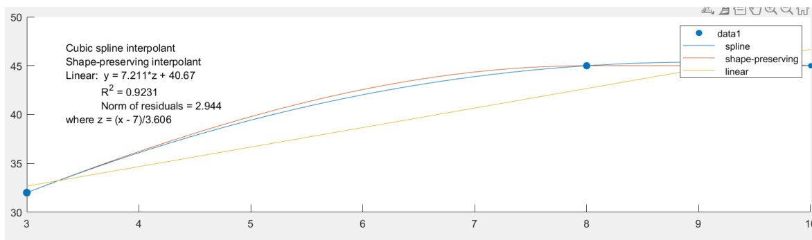
Figure 1. The Effect Size of Ejection Fraction Value < 50% on the BIS Index Value
