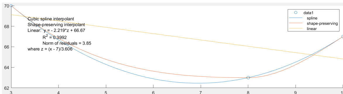
Figure 5. The Effect Size of Ejection Fraction Value < 50% on Heart Rate
