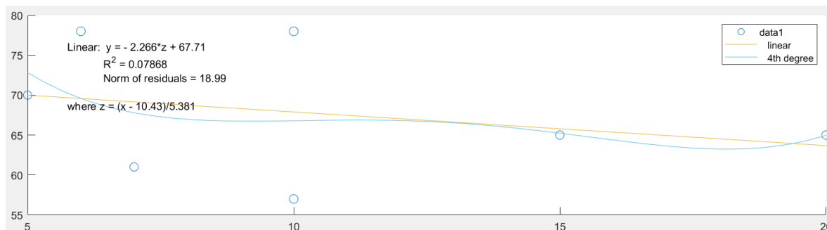
Figure 4. The Effect Size of Ejection Fraction Value ≥ 50% on Mean Arterial Pressure
