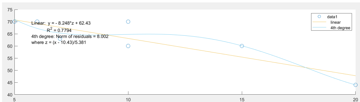
Figure 2. The Effect Size of Ejection Fraction Value ≥ 50% on the BIS Index Value
