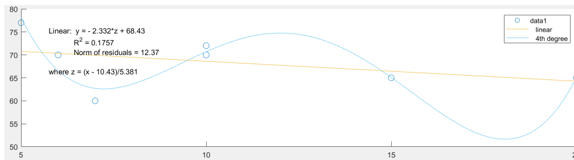
Figure 6. The Effect Size of Ejection Fraction Value \geq 50% on Heart Rate
