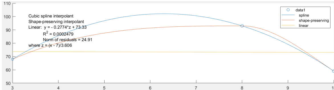
Figure 3. The Effect Size of Ejection Fraction Value < 50% on Mean Arterial Pressure
