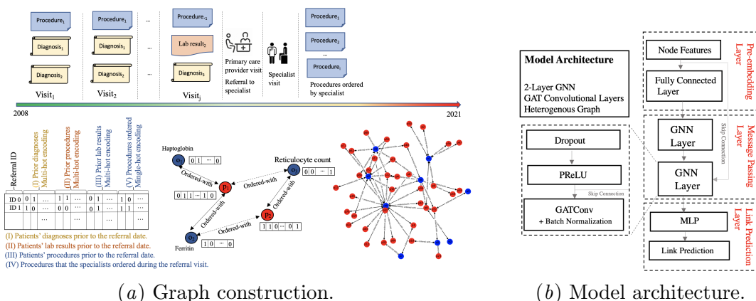
Figure 2: Patients EHR data are formatted in a multi-hot encoding matrix. Red nodes show patients and blue nodes show procedures. Each patient node is assigned with a multi-hot encoded feature vector consisting of the concatenation of diagnoses and lab results features, and each procedure order node are associated with one-hot encoding of the procedure IDs. Solid edges show procedures ordered before referral dates and dashed edges show procedures ordered by specialists and after referral dates (targets).
