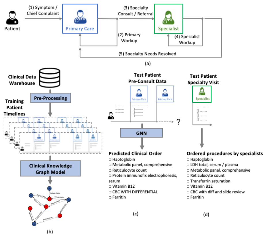
Figure 1: Overall schema of the proposed framework. (a) Specialists' orders and workup can be initiated by primary care providers at referral or consultation time. (b) Patients' historical EHR data including diagnoses, procedures, and lab results were used to create a heterogeneous GNN. Nodes are patients and orders. Solid line edges show orders before referral and dashed line edges show the specialists orders after referral date. (c) The GNN model was used to predict future specialists' orders. This figure shows the GNN model recommendations for one example patient referred to the hematology clinic. (d) Procedures ordered by specialists (ground truth) for the example patient shown in (c). This list highly overlaps with the procedures recommended by the GNN model (c).
