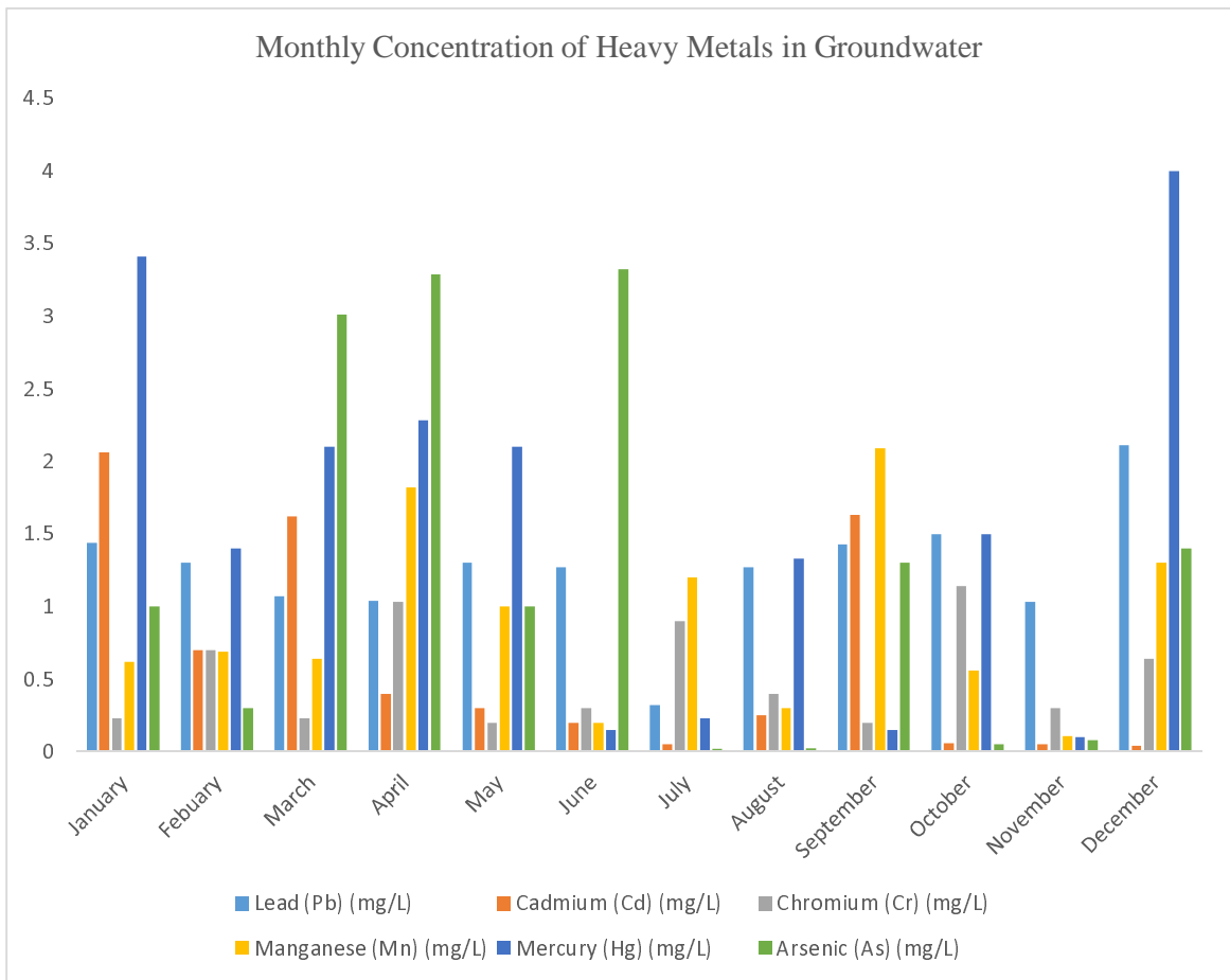
Fig. 17: Monthly variation of Pb, Cd, Cr, Mn, Hg & As in ground water
