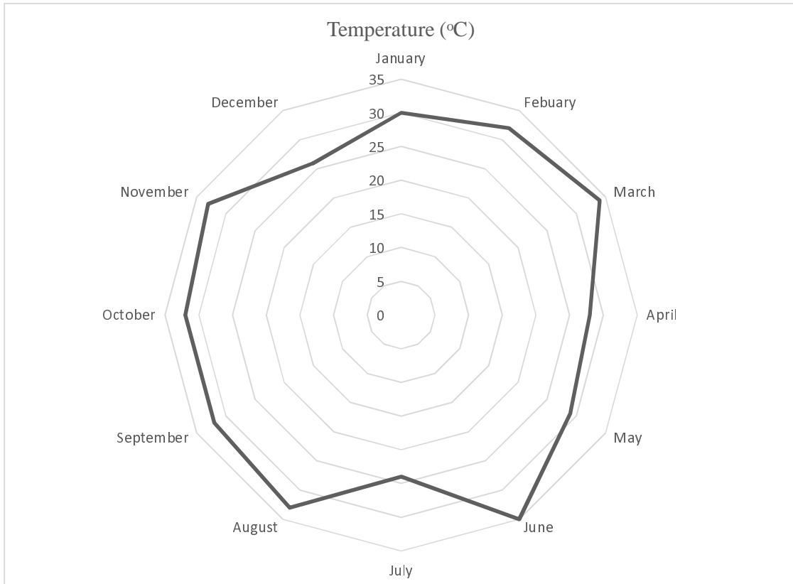
Fig. 14: Monthly variation of Temperature in ground water
