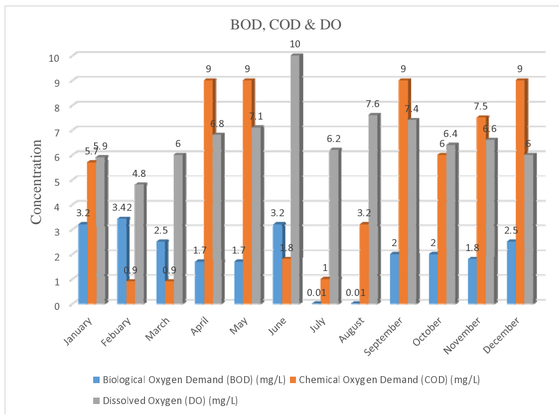
Fig. 9: Monthly variation of BOD, COD & DO in ground water
