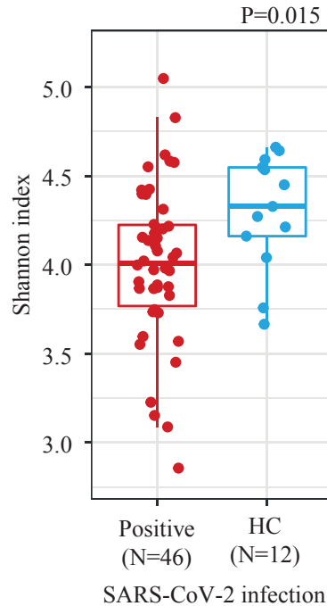
Figure 1. Gut microbial diversity of pregnant women differs by SARS-CoV-2 infection. Alpha diversity is shown using Shannon index comparing pregnant women with SARS-CoV-2 infection during pregnancy vs. pregnant women healthy controls (HC). The statistical test applied was a Linear regression.
