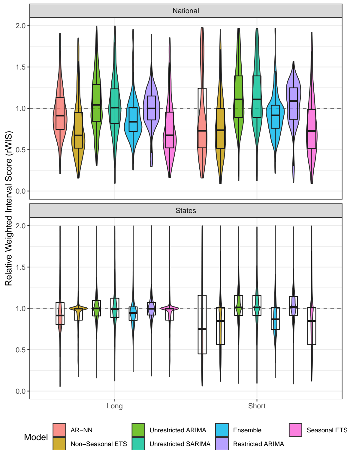
Figure 1: rWIS distributions for each model and training data length for National and State targets across all forecast dates and week-ahead horizons. Distribution is illustrated by a density polygon with a boxplot overlay. rWIS was truncated at 2.0 to aid in visualization, even though some models had extremely high rWIS values for some observations.
