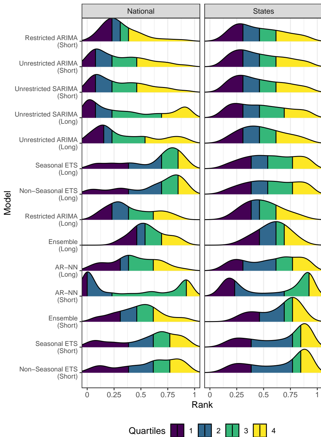
Figure 2: Standardized rWIS rank distribution for each model (and training data length) across locations, forecast dates, and horizons. A standardized rank of 1 indicates that the model had the lowest (best) rWIS across locations, targets, and forecast horizons, and a standardized rank of 0 indicates that the model had the worst (highest) rWIS. The quartiles of each model’s distribution of standardized ranks are shown by different colors with yellow indicating the top quartile and indigo representing the bottom quartile of the distribution. Models are ordered by model with the lowest median rWIS on the bottom to the highest median rWIS on the top, averaged across states and national targets.
