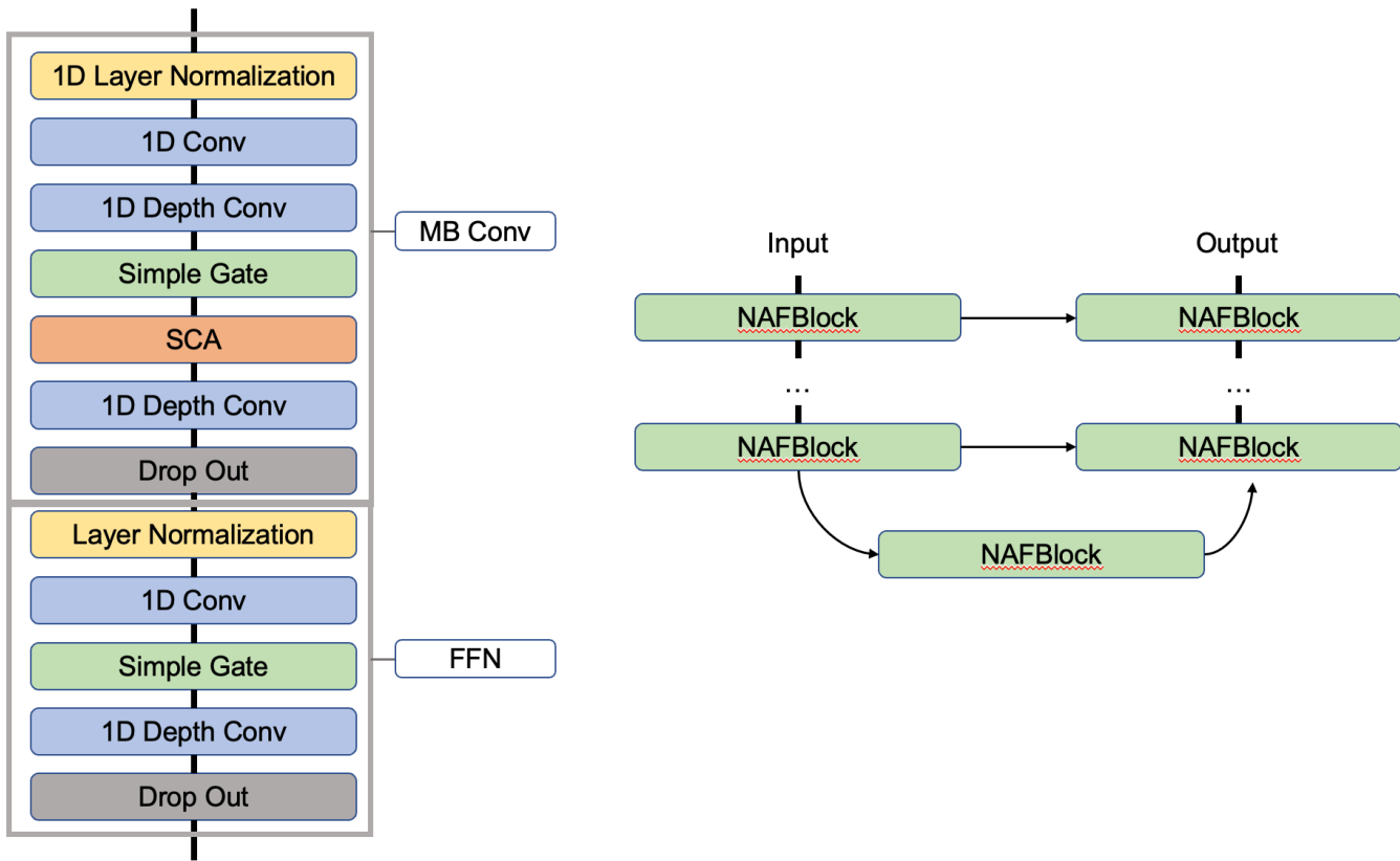
Figure 1: Figure 1a describes the structure of the Block using Mobile Convolution (MB Block) and Feed Forward Network (FFN) Block with changes to the attention layers using simple channel attention (SCA) and simple gate along with drop out layers. Figure 2b describes the overall U-shaped architecture of Cardio-NAFNet where the left side represents encoder with 10 NAFBlocks and the right side is the decoder with 4 NAFBlocks. The decoder also receives maps from the encoder blocks using skip connection.
