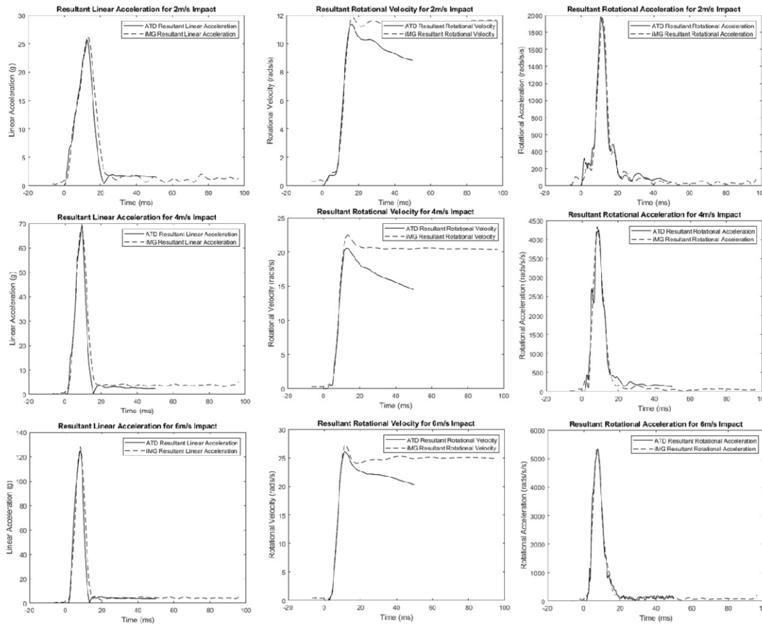
Figure 2: Examples of the ATD (solid line) and iMG (dashed line) measured head kinematics. The curves are synched using the peak values and then used to calculate RMS and NRMS errors. Column 1 represents linear acceleration curves, column 2 rotational velocity curves, and column 3 rotational acceleration curves. Row 1 represents a 2m/s impact, row 2 a 4 m/s impact, and row 3 a 6 m/s impact.
