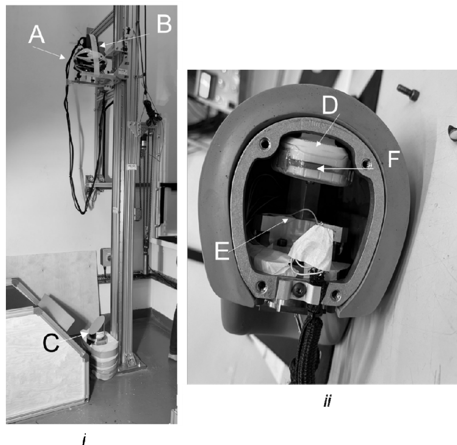
Figure 1: i ) the testing drop rig: A = helmet, B = headform, C = Anvil. (ii) the Hybrid III headform, with mouthguard placement: D = plastic teeth, E = 9-accelerometer array, F = mouthguard.
