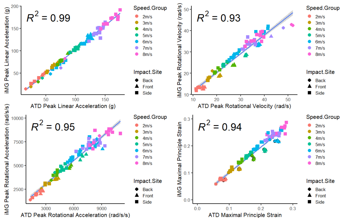
Figure 3: Scatter plots for peak linear acceleration, peak rotational velocity, peak rotational acceleration and maximal principal strain, measured by the ATD and iMG. Linear regression trendline ( \pm 95\% CI on line) and R squared values displayed on each graph.
