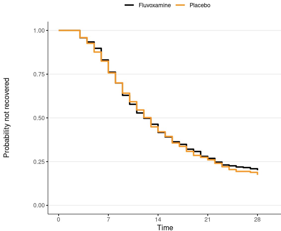
Figure 3. Kaplan-Meier for primary outcome of time to sustained recovery
