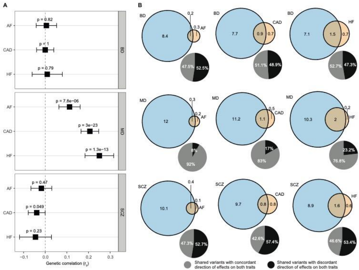
2 3 Figure 1. MD exhibits significant genetic correlation and polygenic overlap with CVDs. (A) 4 Genetic correlations ( r_g ) between the three psychiatric disorders and three CVDs analysed in this 5 study. The dotted line indicates a lack of genetic correlation ( r_g = 0 ). Error bars indicate 95% 6 confidence interval for the r_g estimates, and the corresponding p-values are shown. (B) Polygenic 7 overlaps between psychiatric disorders and CVDs. The Venn diagrams show the number 8 (thousands) of trait-associated variants specific to each psychiatric disorder (blue), specific to each 9 CVD (yellow), and shared by a pair of psychiatric disorder and CVD (overlap), as estimated by 10 MiXeR. The pie charts show the percentages of shared variants (corresponding to the overlapped 11 region in the relevant Venn diagram) that confer concordant (grey) and discordant (black) 12 directions of effects on both traits. AF, atrial fibrillation; BD, bipolar disorder; CAD, coronary 13 artery disease; CVD, cardiovascular disease; HF, heart failure; r_g , genetic correlation; MD, major 14 depression; SCZ, schizophrenia.
