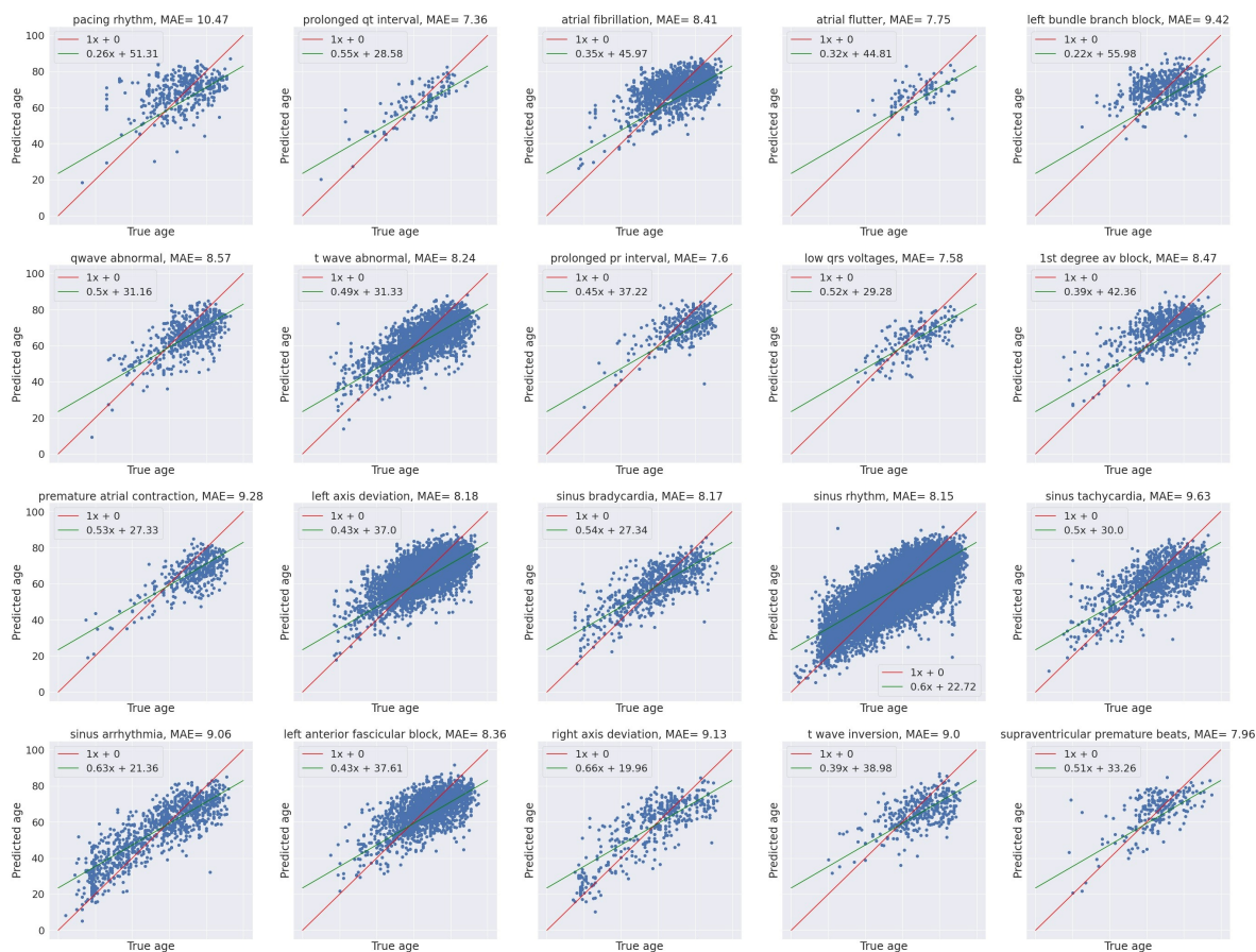
Figure 5: Predicted age from the Inception Time model versus true (biological) age of the patient in the test set. The comparison of predicted and true age are categorized into 20 groups of different cardiovascular conditions.
