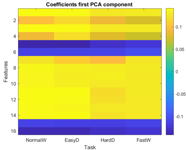
238 239 Figure 3. Contribution of the 16 STGF in each task to the first PCA component.
