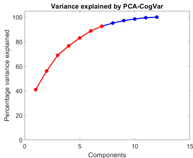
246 247 Figure 4. The cumulative sum of the variance accounted for the 12 PCA components.
