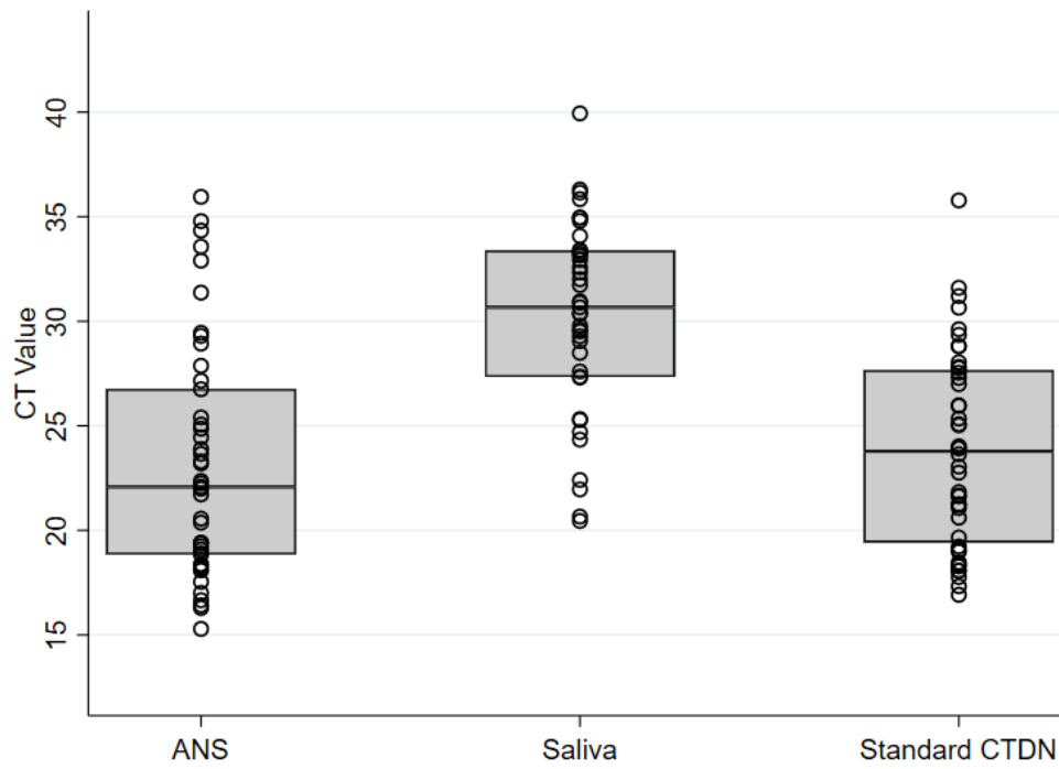
Figure 1: Distribution of CT-values for E-gene among all sampling methods
