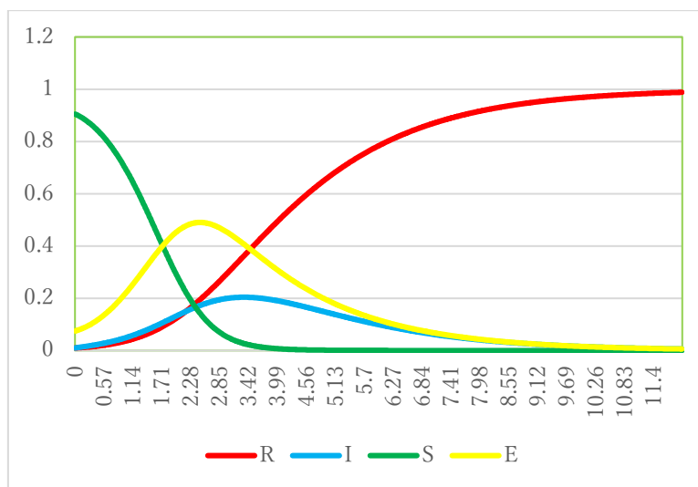
Fig.1. Four curves for S(t), E(t), I(t) and R(t) with \beta = 10, \gamma = 1 and \sigma = 0.5 .
