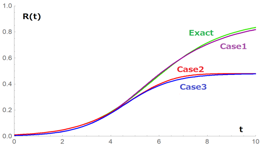
Fig. 2 Curves of approximate solutions for Cases 1, 2 and 3, against the Exact equation solution. The Case 3 is for the logistic equation.
