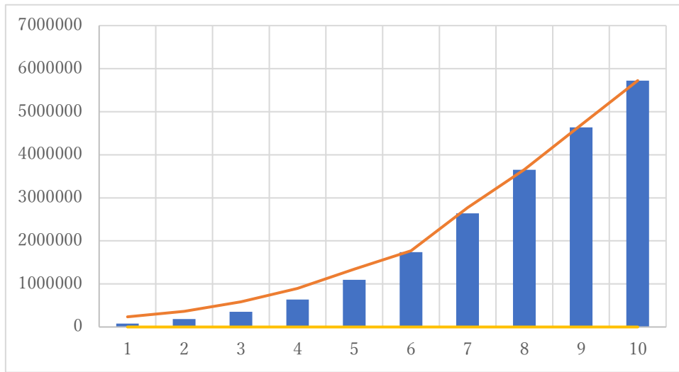
Fig. 3. The red line shows a curve of R(t) with \alpha = 10 , \gamma = 1 and \sigma = 0.5 . Blue bar charts stand for the 7th-wave data of R(t) .
