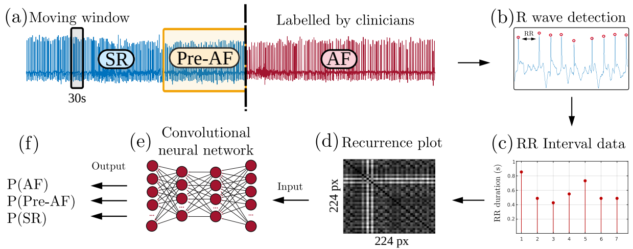
Figure 2. Pipeline of the first stage of AFiRMo. (a) Each ECG record is split into three classes: SR, Pre-AF, and AF. (b) R peaks are detected from a sliding window of 30s in the ECG data. (c) RRI signal is generated from the R peaks. (d) A recurrence plot is generated from the RRI signal. (e) A deep CNN is trained using the recurrence plots as inputs. (f) Network output are the probabilities of the sampled data to belong to each of the three classes (SR, Pre-AF, and AF).
