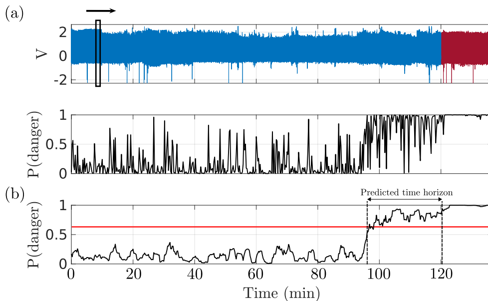
Figure 3. Second stage of AFiRMo: indicator of early warning. (a) Probability of danger computed by AFiRMo as a function of time for a representative patient from the test dataset. The sample images are generated by taking a sliding window of 30s every 15s and the probability of danger is computed for every sampled window. (b) Average probability of danger, computed from a non-anticipative moving average window of 7 samples to smooth the probability fluctuation. The red line is a threshold of 0.57 that will trigger a warning of an imminent AF onset.
