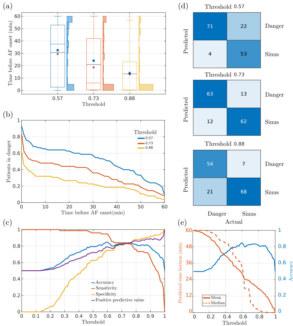
Figure 4. Performance of AFiRMo with 7 samples moving average. (a) Box plots of the predicted time horizon until AF onset for different probability thresholds across all patients. Median and mean values are marked by coloured and black lines, respectively. Blue circles and red asterisks represent the means of patients younger and older younger than 65 years, respectively. Histograms of the predicted time horizon are shown on the right side of the box plots. (b) Fraction of patients predicted to be in danger as a function of time before the AF onset for different thresholds. (c) Performance metrics as a function of the probability threshold. (d) Confusion matrices for different values of the threshold. (e) Mean (solid line) and median (dashed line) of the predicted time horizon and model accuracy as a function of the probability threshold.
