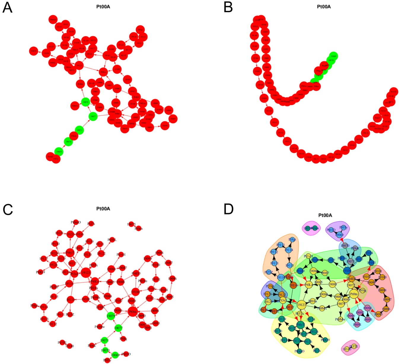
Figure 6: Point-based chronological graph of one frequently repeated location. A, source chain graph of the point Pt00A; B, target chain graph of the point Pt00A; C, source chain plus target points of the point Pt00A modified by rescale the vertex size by degree of connection; D, full chain of the point Pt00A clustered by community (connection density) via random walk;
