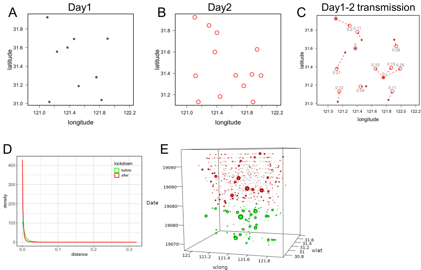
Figure 3: The point-wise viral spreading based upon the day-to-day nearest neighbour assumption. A-C, represent the toy data of point-wise day 1, day 2 and day-to-day viral transmission assumption; the point-wise nearest neighbour distance from the day 1 to day 2 was estimated by set the day 1 locations of reference as a whole and search the nearest neighbour of the locations of the day 2 point-by-point; D, the distribution of the nearest neighbour distance, the distance from the repeated address in second day to that of previous day was zero; E, visualize of the spatial distribution of nearest neighbour distance with sphere radius proportion to the estimated distance in the periods of before lockdown (green sphere for freeTransp) and city total lockdown (red sphere for tLockdown);
