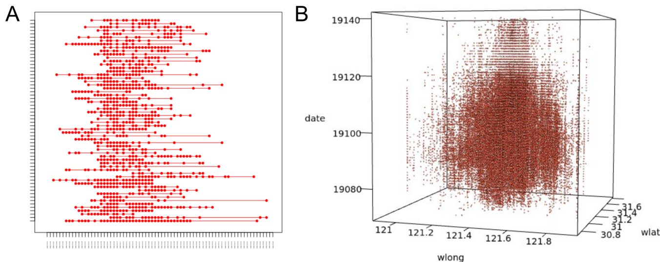
Figure 4: Example of pattern of repeatedly reported locations. A, Example of the repeated locations along the date; B, Examples of the repeated locations along the date with longitude and latitude;
