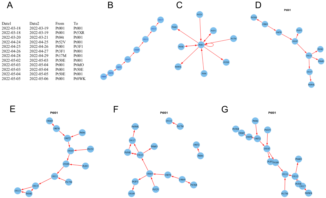
Figure 5: To generate directed acyclic graph by combining spatio-temporal data. A, a toy dataset; B, chronological sequence of specific point and the date was converted into integer dated from the origin of 1970-01-01; C, the directed acyclic graph of specific point; D, graph combining specific point as source of transmission and its chronological sequence (source chain); E, graph combining specific point as target of transmission and its chronological sequence (target chain); F, graph combining specific point both as source and target of transmission and its chronological sequence (source chain plus target points); G, graph combining the chronological sequence and both as source and target of transmission (full chain);
