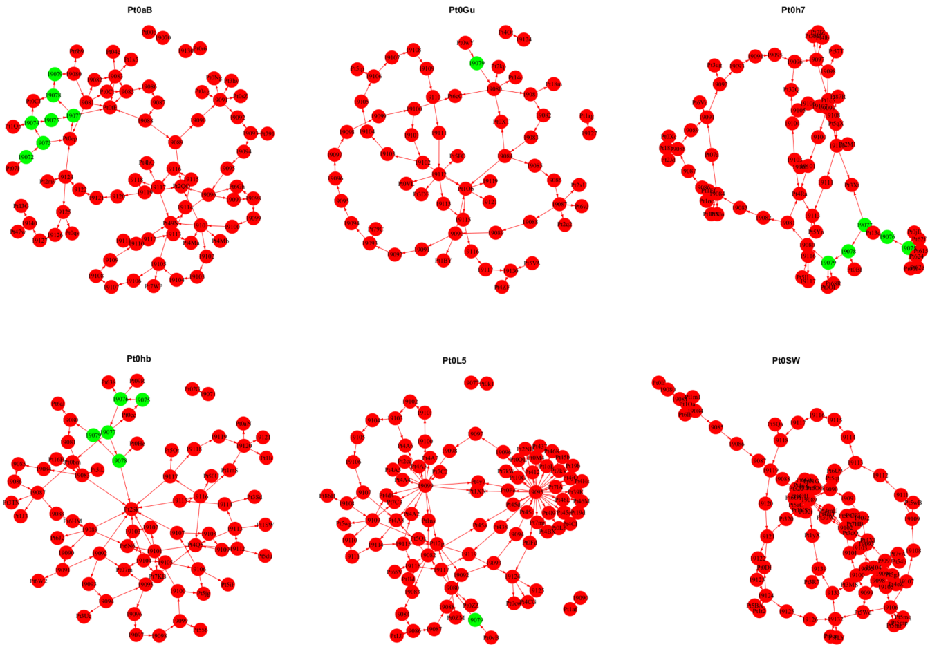
Figure 7: Some commonly appeared locations as source based upon the day-to-day nearest neighbour transmission assumption (green and red nodes represented date before and after the city lockdown, respectively).
