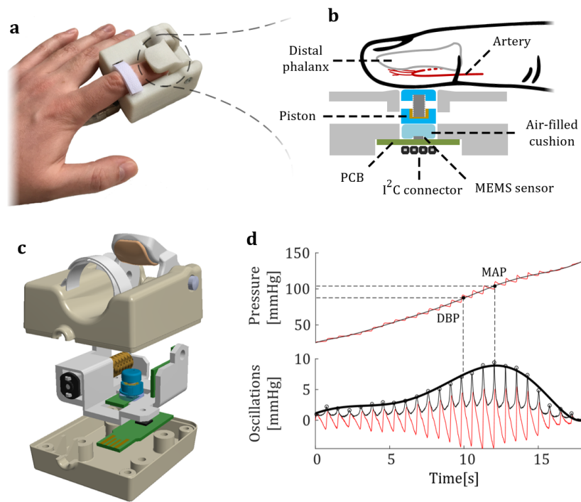
Fig. 1. Instrument overview. a) Photograph showing the device in use. b) Cross-sectional view of the sensor setup. c) 3D model of the device. d) Oscillometric method. The pressure ramp signal is filtered with a pass-band filter (1 - 10 Hz) and Hilbert transformed. The peaks, or oscillations, are detected, and a polynomial curve is fitted to the peaks. The resulting bell-shaped curve is called an oscillometric waveform envelope (OMWE). Mean arterial pressure (MAP) is found at the point on the pressure curve that corresponds with the maximum of OMWE. DBP is found on the left side of the OMWE at 80% of maximum pressure. SBP is computed from DBP and MAP.
