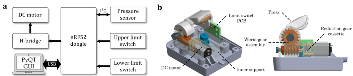
Fig. 2. Description of the system. a) Block diagram of the system. An ARM Cortex M4 based MCU is used as the controller unit. The MCU is connected to a laptop running a Python GUI for data logging. b) Inner mechanics illustrated in a 3D view. A DC motor is connected to a worm gear assembly through a reduction gear cassette. This rotates a hinge-type press that is used to apply pressure to the finger. A pair of micro limit switches assembled on a custom circuit board is used to limit the motion.
