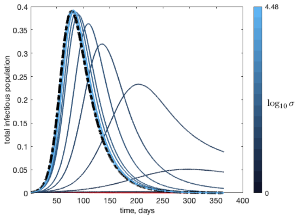
Fig. 2. As \sigma \rightarrow \infty , the pair model approaches the standard SIR model with mass action. The black broken line shows the total number of infections for the SIR model and the solid lines show the total infections over time as \sigma gets large.
