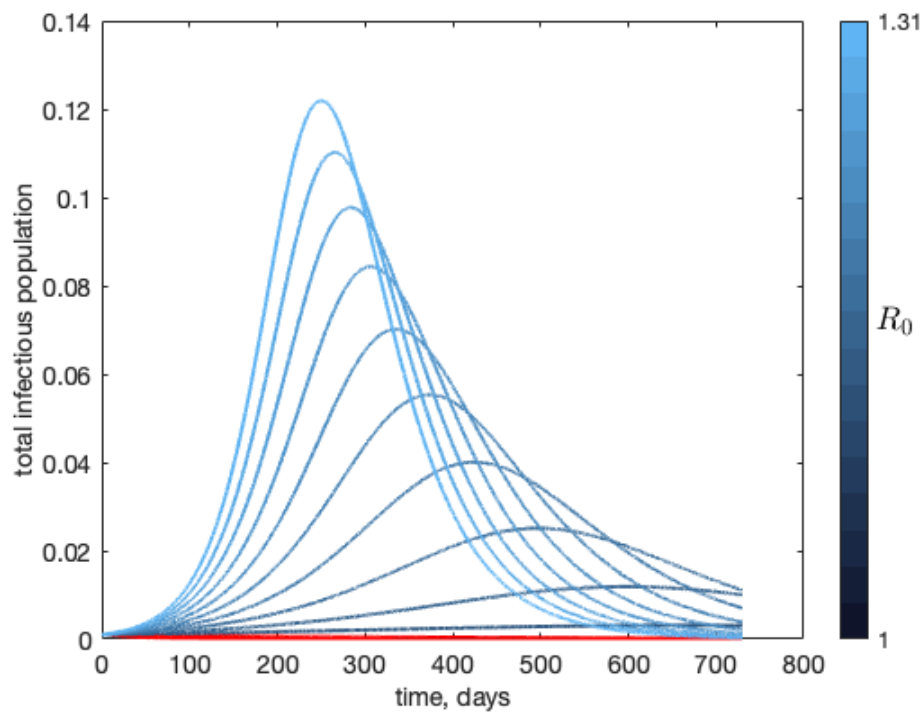
Fig. 3. The different outcomes of an outbreak as a function of R_0 . The total infectious population, I + P_{SI} + 2P_{II} + P_{IR} , is shown for a range of R_0 , from 1 to 1.31.
