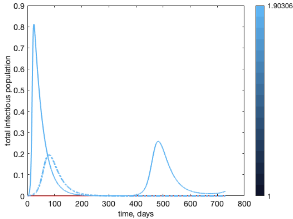
Fig. 5. A comparison of the pair formation model (equations Eq. (1) to Eq. (9)) with an SIR model with standard incidence (equations Eq. (11) to Eq. (13)). Parameters for both models are chosen so that R_0 = 1.9 for both models.
