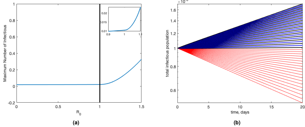
Fig. 1. Numerical confirmation of R_0 (equation Eq. (20)), visualized in two ways. We start all simulations with I(0) = 1 \times 10^{-3} . Panel (a): The maximum number of infections for the model given by equations Eq. (1) through Eq. (9) as a function of R_0 . We see that the expression for R_0 provided by equation Eq. (20) is verified numerically. Panel (b): Infection curves for different values of R_0 . Red curves represent where R_0 < 1 and black/blue curves are scenarios where R_0 > 1 . Colours alternate between black and blue for clarity.
