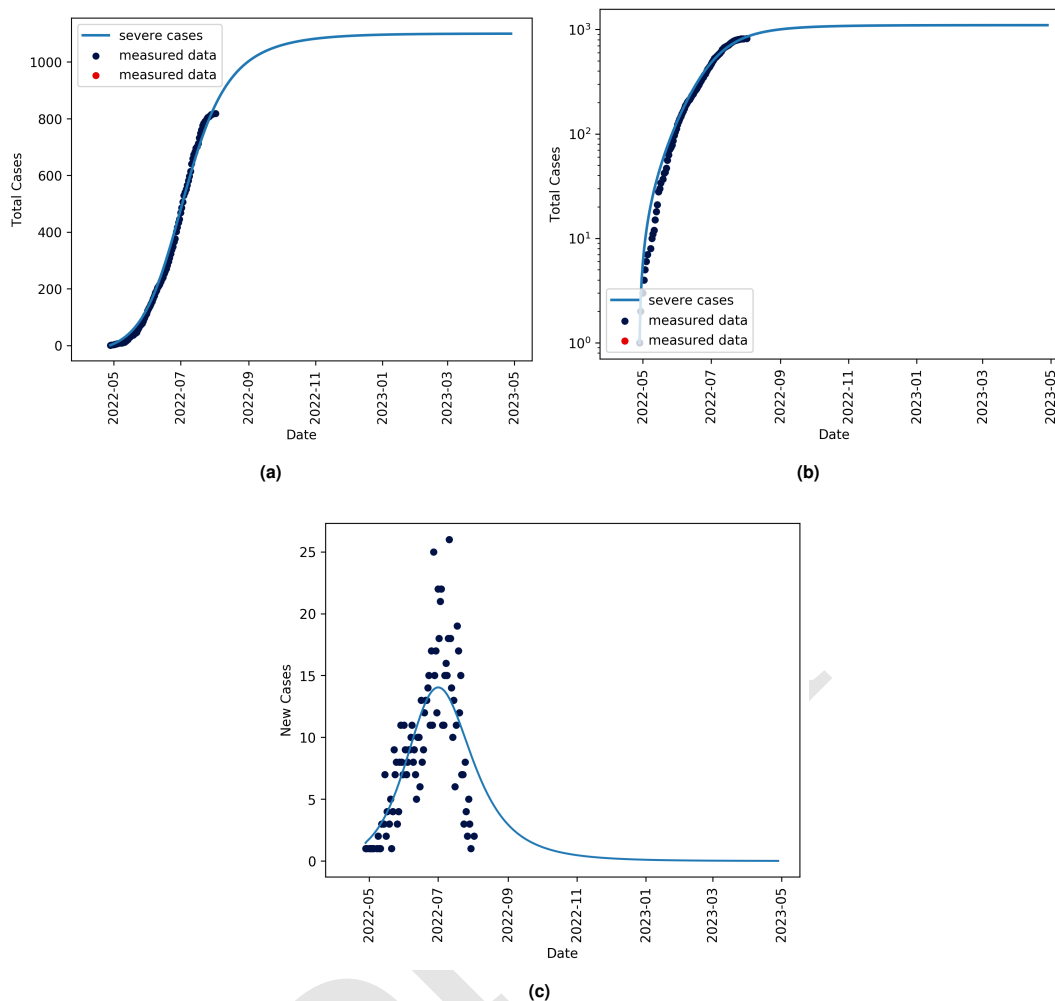
Fig. 6. Curves for cumulative infections in Canada on a linear scale (a) and log scale (b) for clarity. Panel (c) shows the new cases per day. Canadian data is taken from (29) and fits are generated using equations Eq. (1) to Eq. (9).
