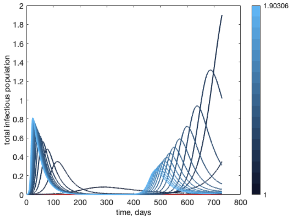
Fig. 4. Multiple waves of infection. The total infectious population, I + P_{SI} + 2P_{II} + P_{IR} , is shown for a range of R_0 . Pair formation coupled with the ability to recover from infection leads to multi-wave dynamics.
