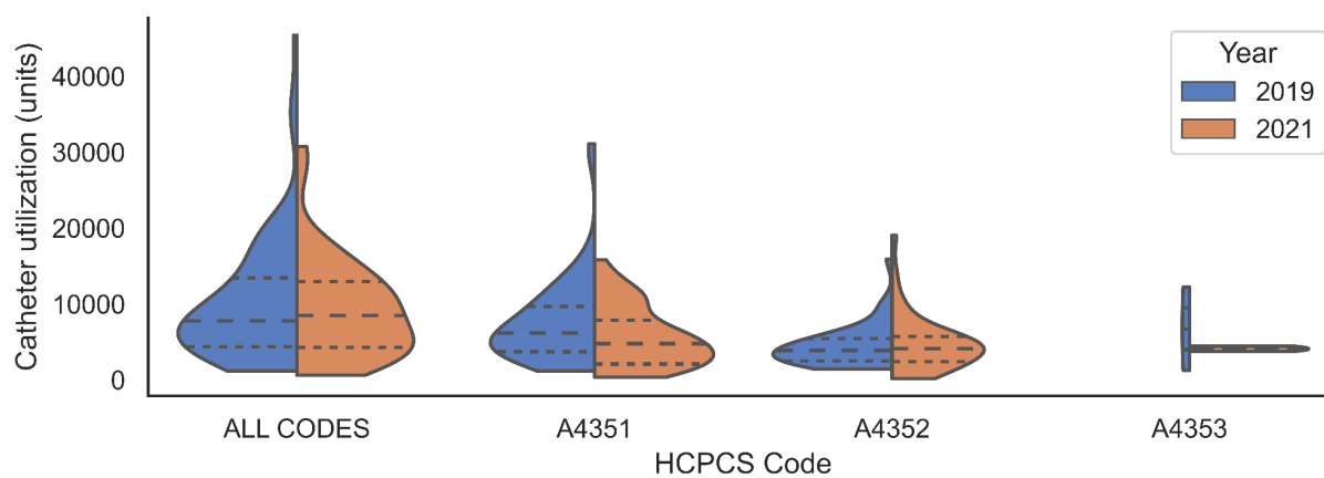
Figure 5. Violin plot of catheter utilization by referring providers, comparing 2019 Medicare part B claims against 2021 Medicare and commercial claims for physician-managed services. Dashed lines represent quartiles.
