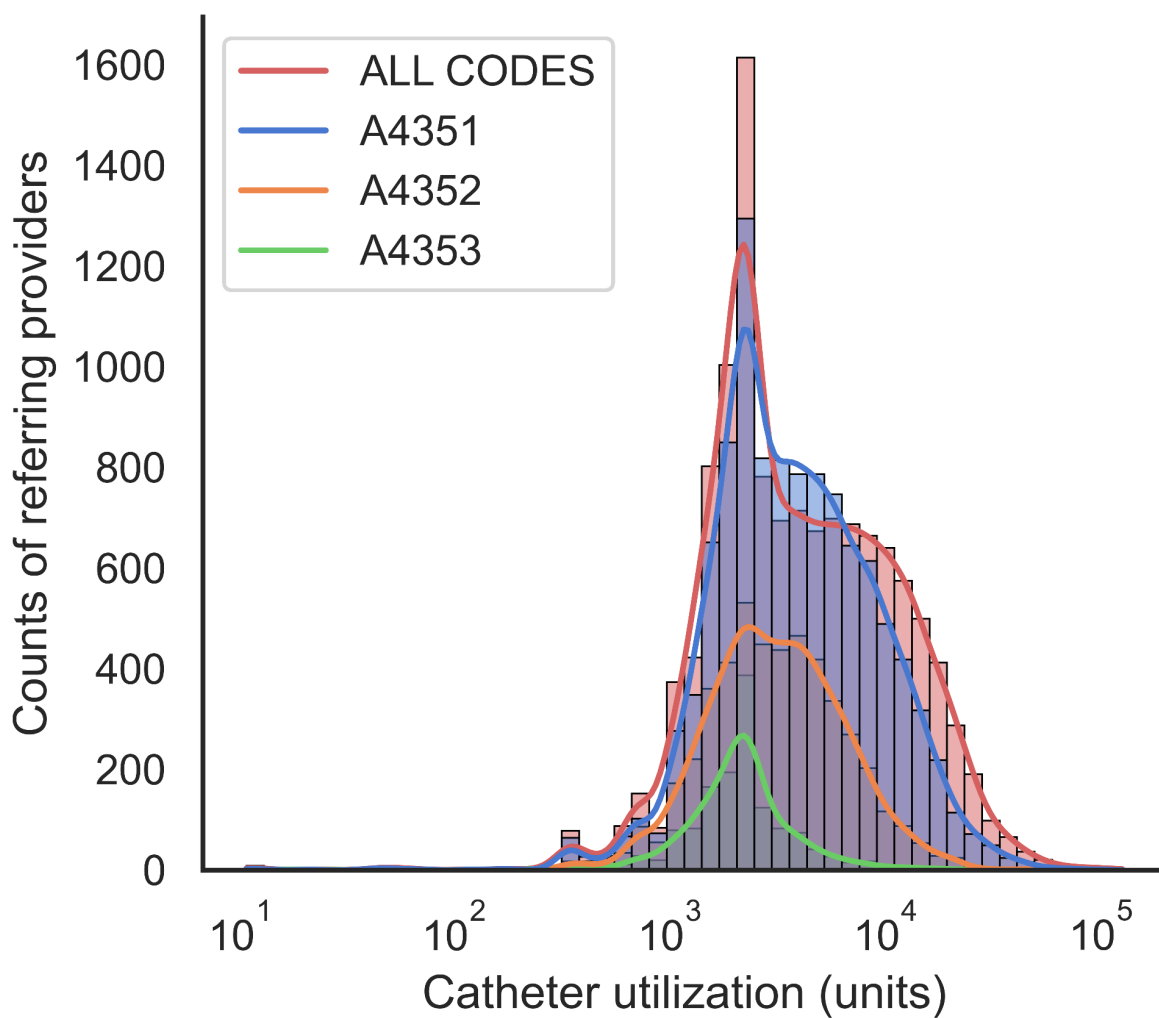
Figure 2. Histogram of referring provider counts (and kernel density estimate) binned by catheter utilization for 2019 Medicare part B claims. The distribution of data for 2019 is representative of other years observed in this study.
