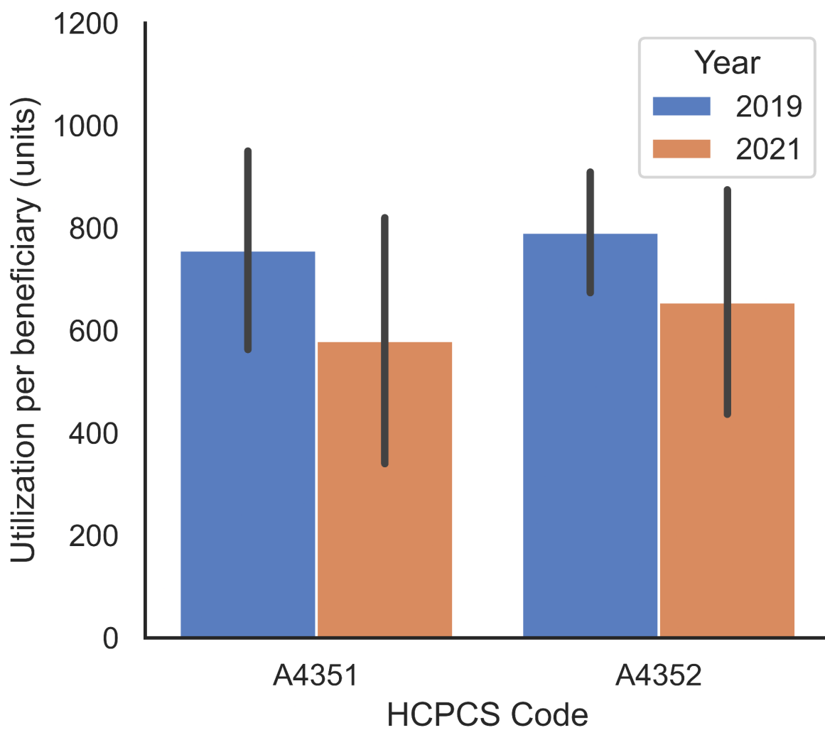
Figure 6. Median utilization per beneficiary (+/- 1 S.D.) for HCPCS codes A4351 and A4352, comparing 2019 Medicare part B claims against 2021 Medicare and commercial claims for physician-managed services.
