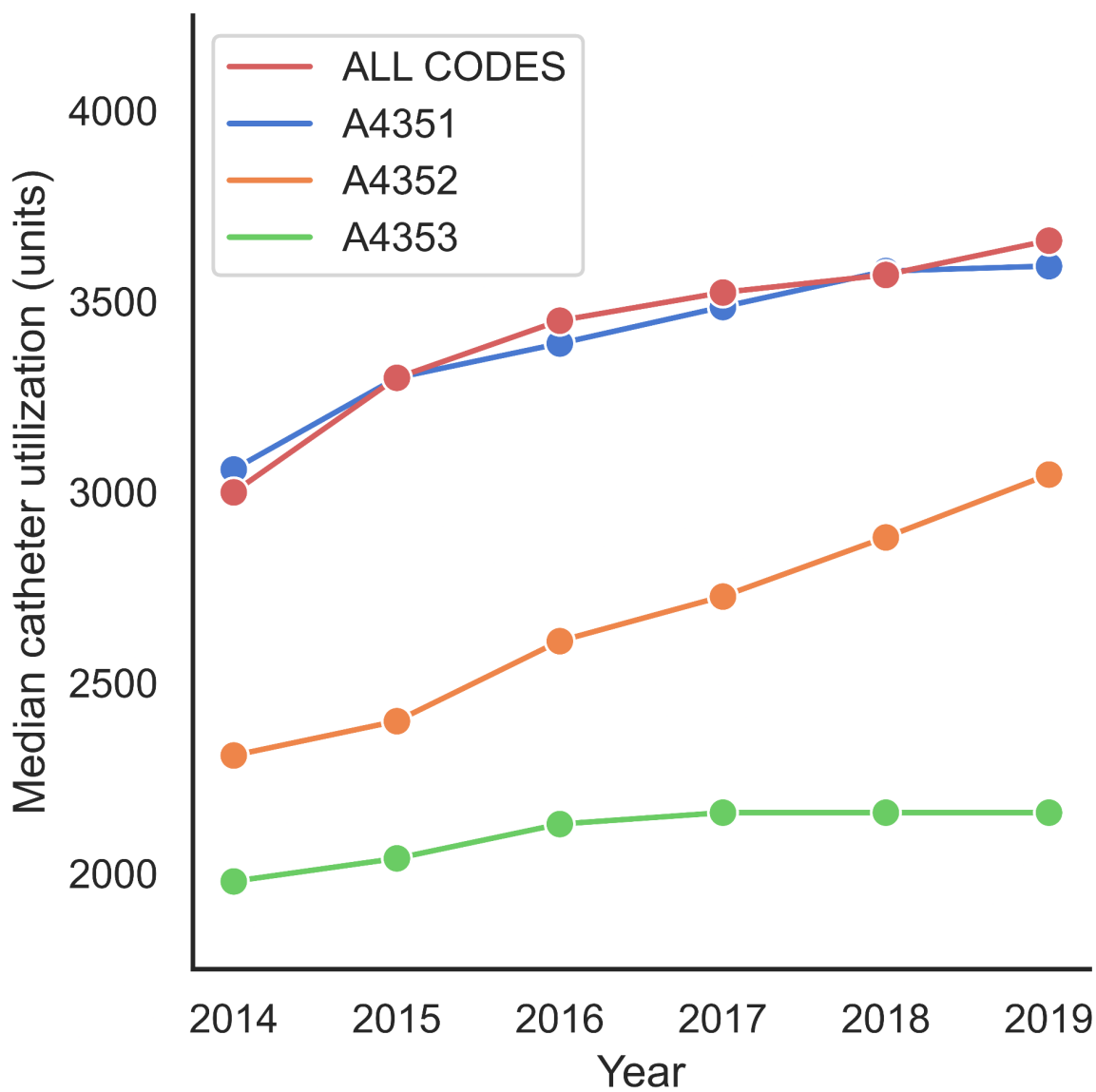
Figure 1. Median utilization of catheters per provider by HCPCS code from Medicare part B claims data.
