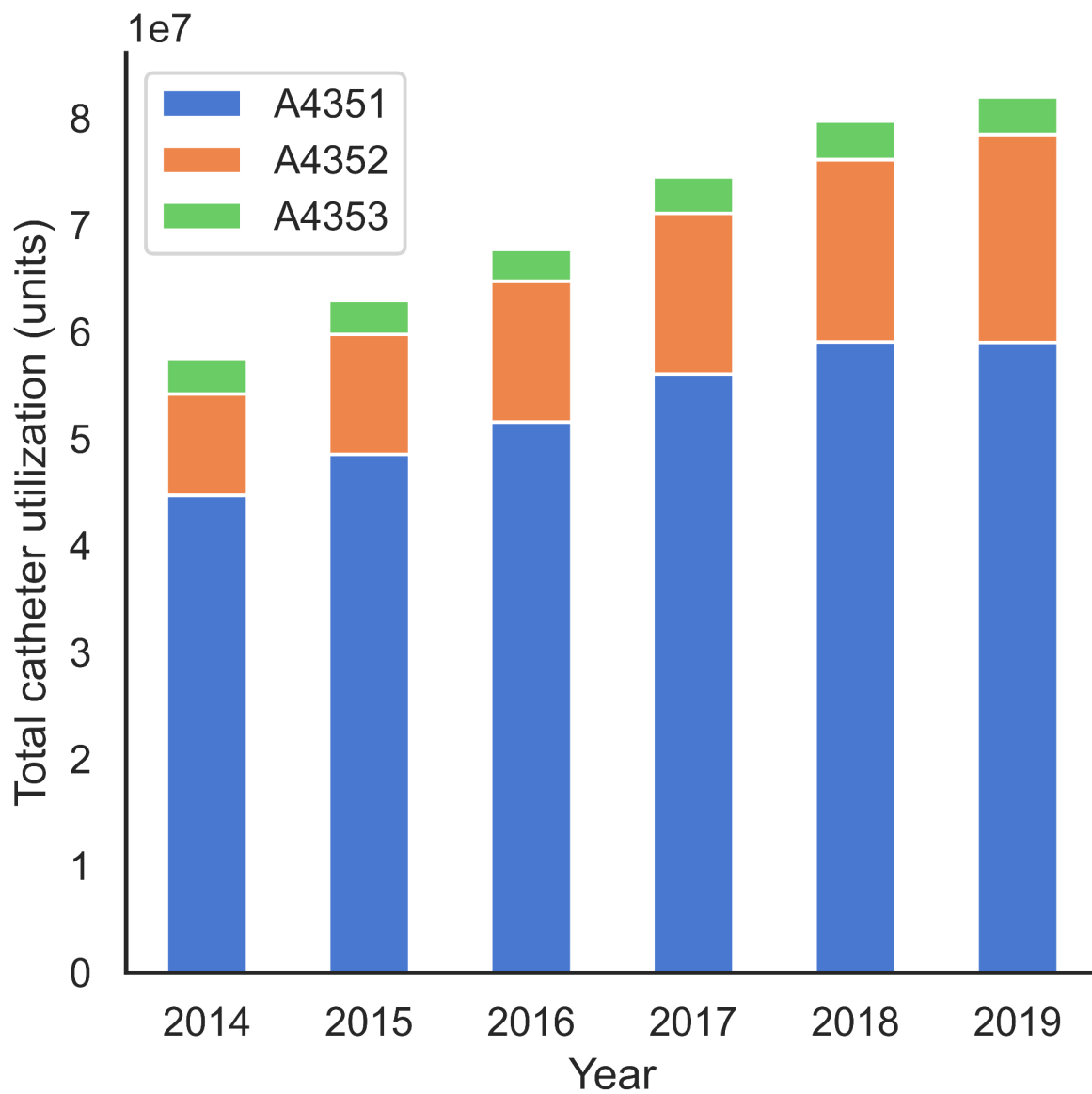
Figure 3. Total utilization of urological catheters by HCPCS code from Medicare part B claims data.
