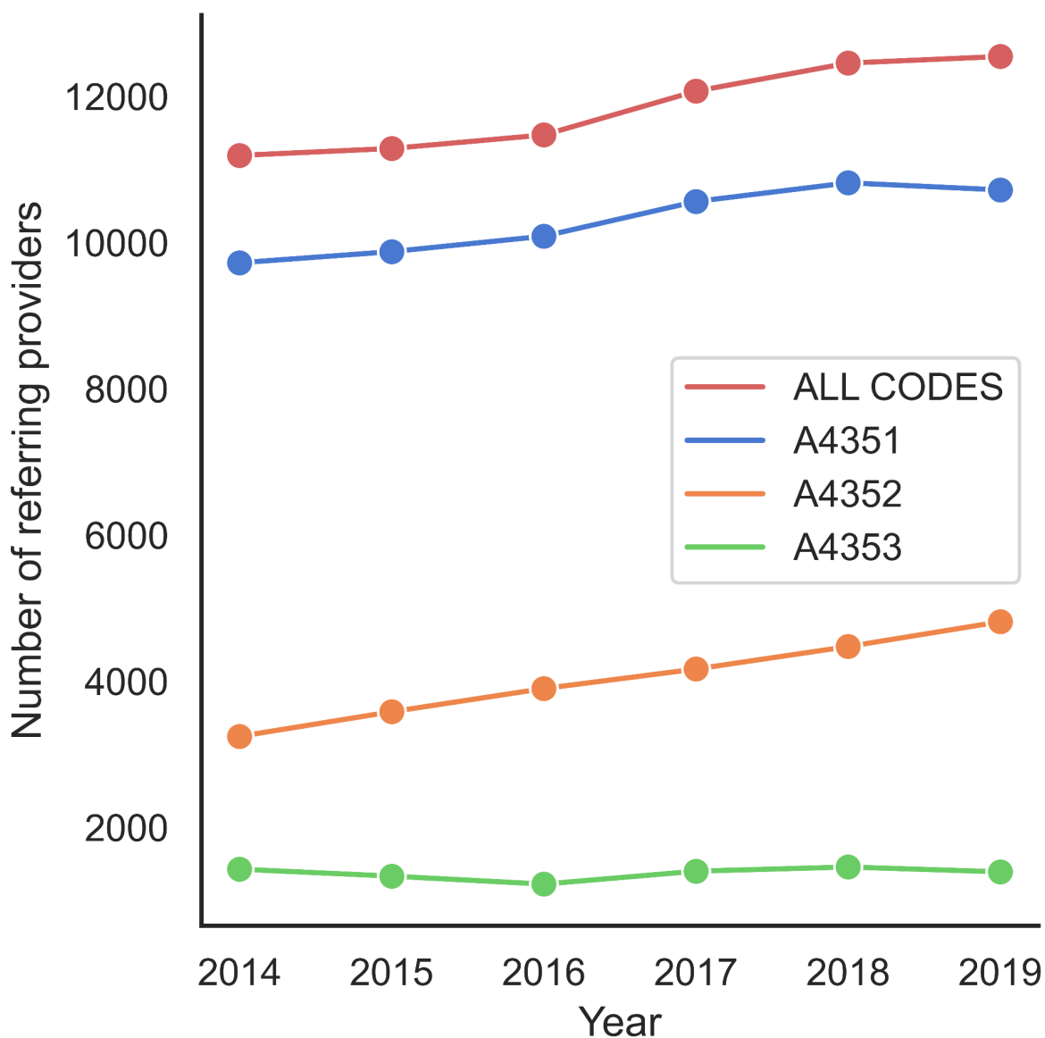
Figure 4. Number of referring providers who utilized catheter HCPCS codes A4351, A4352 and/or A4353 from Medicare part B claims data (a given provider may utilize one or more HCPCS code in a particular year).
