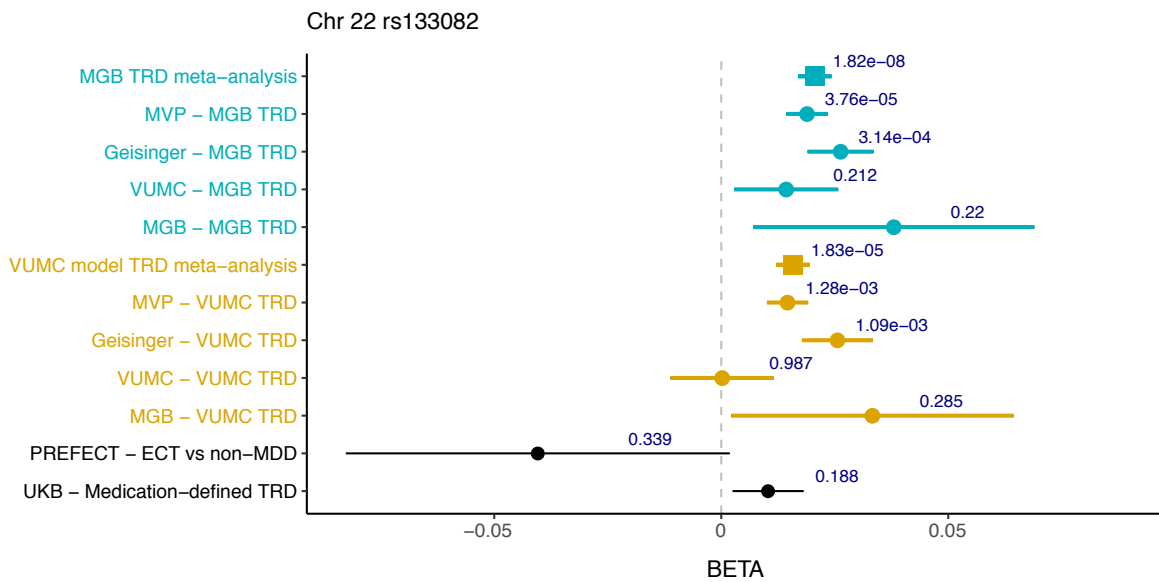
Figure 3: Forest plot of the genome-wide significant locus rs8050136 on chromosome 16 and rs133082 on chromosome 22. The points indicate the log odds ratio and the error bars show the standard error. The P value of association with each phenotype is shown above the error bars.
