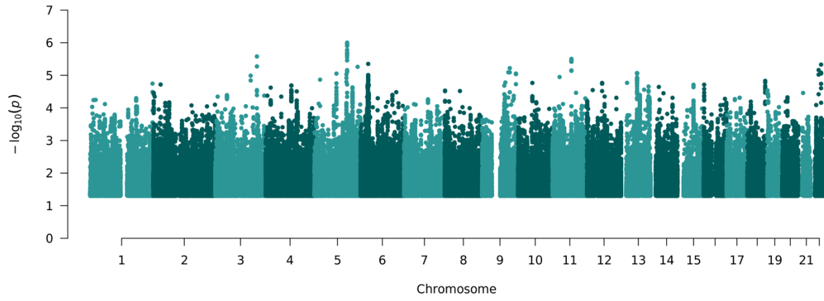
Figure 2: Manhattan plots of A. MGB TRD meta-analysis and B. VUMC TRD meta-analyses
