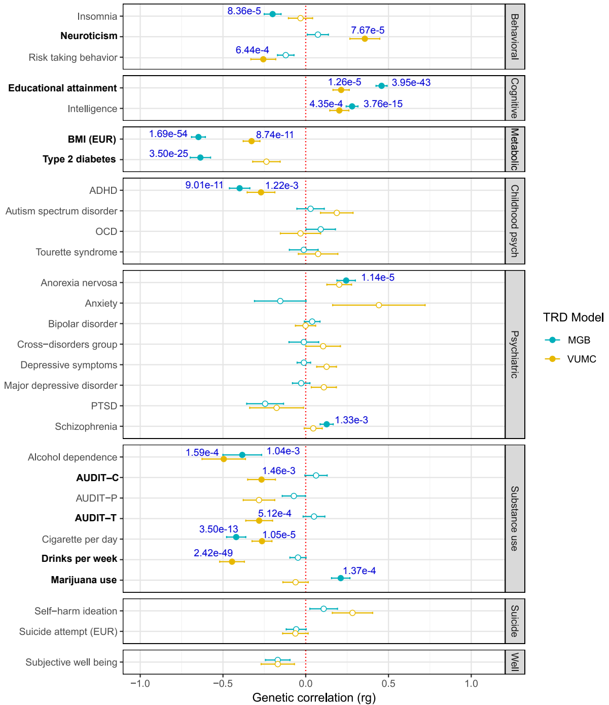
Figure 4: Genetic correlations of VUMC and MGB TRD meta-analyses with psychiatric and non-psychiatric traits. Unfilled points indicate genetic correlations that did not pass the Bonferroni-corrected significance threshold P < 1.72 \times 10^{-3} (29 traits tested). Error bars represent the standard error. P values indicate significance after Bonferroni correction. Bolded traits show significant differences in genetic correlations between the two meta-analyses. BMI-body mass index, ADHD-attention-deficit/hyperactivity disorder, OCD-obsessive compulsive disorder, PTSD-post-traumatic stress disorder, AUDIT-C-Alcohol Use Disorders Identification Test-C (measure of quantity of alcohol consumption), AUDIT-P- measure of problematic consequences of drinking, AUDIT-T-total score of AUDIT.
