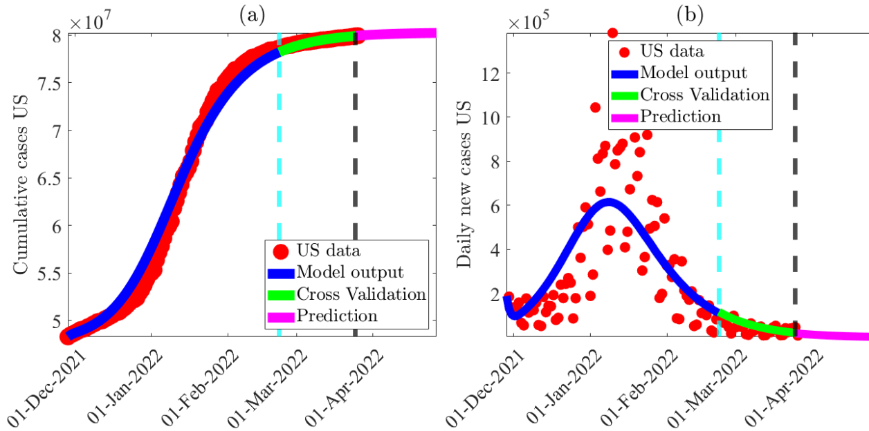
Figure 2: (a) Time series illustration of the least squares fit of the model (2.1), showing the model’s output for the cumulative daily cases in the United States (blue curve) compared to the observed cumulative confirmed cases for the United States (red dots) from November 28, 2021 to February 23, 2022 (segment to the left of the dashed vertical cyan line). (b) Simulation result of (2.1), showing observed daily confirmed COVID-19 cases for the United States as a function of time, using the fixed and estimated baseline parameter values given in Tables 5, 3 and 4, respectively. The segment from February 24, 2022 to April 30, 2022 (i.e., solid green and magenta curves or the entire segment to the right of the dashed cyan vertical line) illustrates the performance of the model (2.1) in predicting the cumulative and daily cases in the United States.
