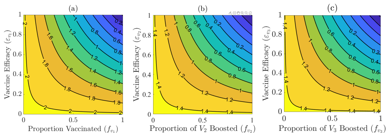
Figure 3: Contour plots of the vaccine reproduction number ( \mathbb{R}_v ) of the model (2.1), as a function of vaccine coverage or boosting at steady-state ( f_{v_i} ; i = 1, 2, 3 ) and vaccine efficacy ( \varepsilon_{v_i} ; i = 1, 2, 3 ), for the United States. (a) Vaccination of wholly-susceptible individuals ( S(t) ; f_{v_1} is proportion of wholly-susceptible individuals who are fully-vaccinated at steady-state). (b) Boosting of vaccinated individuals with moderate vaccine-derived immunity ( V_2(t) ; f_{v_2} is the proportion of vaccinated individuals in the V_2 class who are boosted). (c) Boosting of vaccinated individuals with low vaccine-derived immunity ( V_3(t) ; f_{v_3} is the proportion of vaccinated individuals in the V_3 class who are boosted). Parameter values used in these simulations are as given by their respective baseline values in Tables 3-5.
