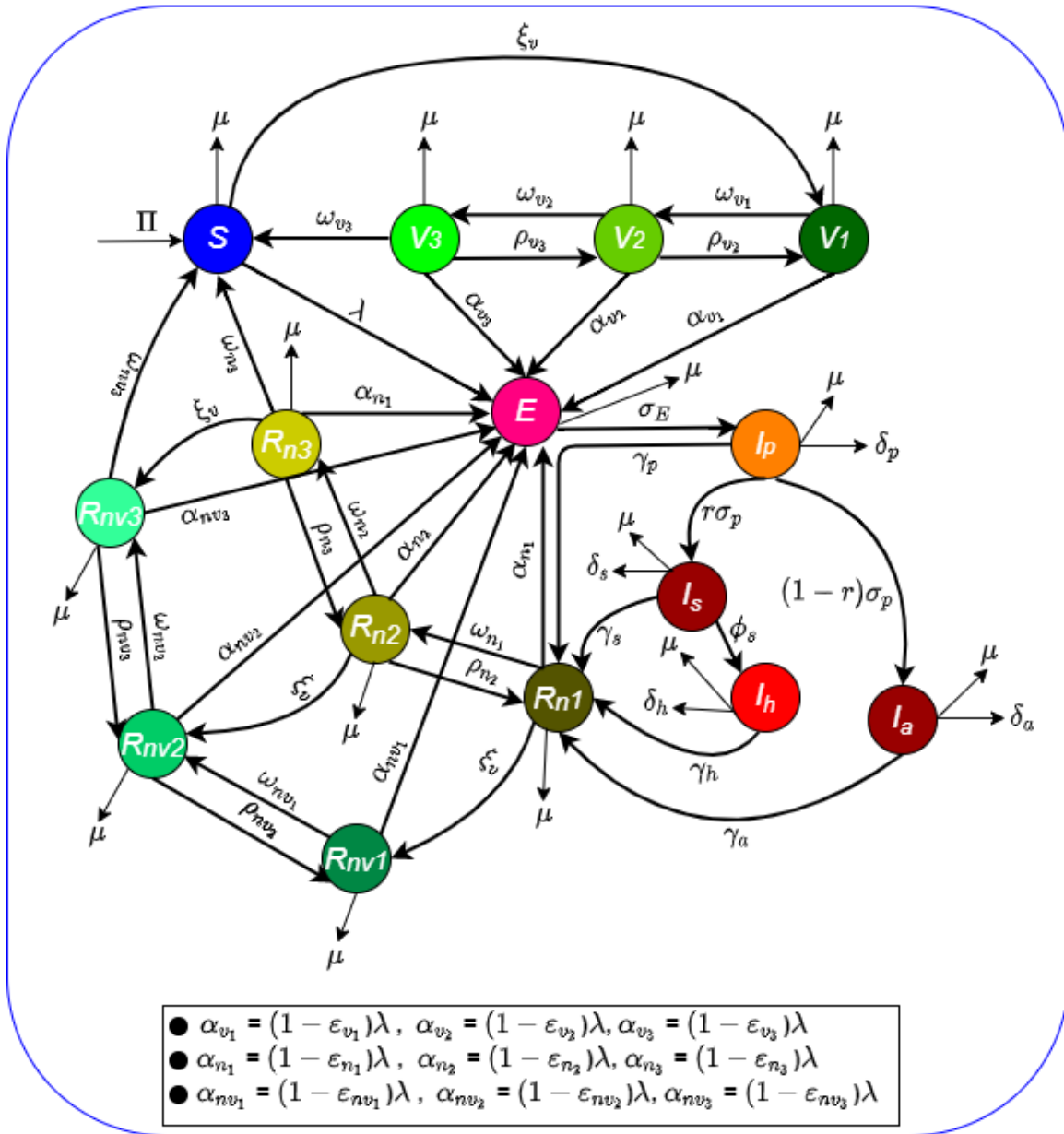
Figure 1: Flow diagram of the model (2.1).
