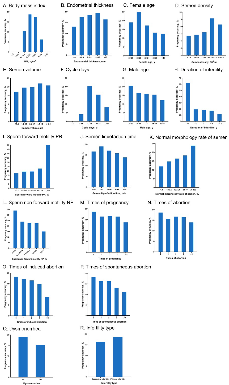
Figure 2. Interval Division Results of 18 Indicators
