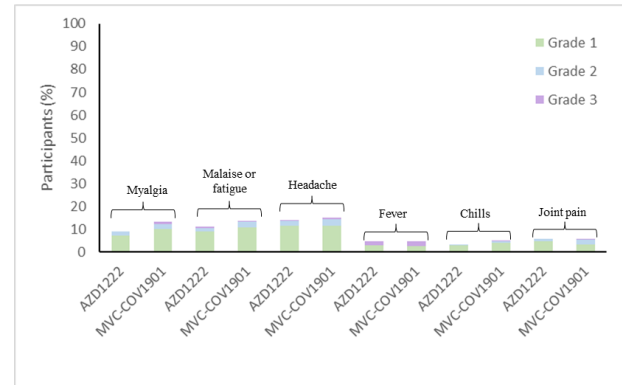
6 Figure 2. Solicited local (A) and systemic (B) adverse events occurring within 7 days of the first 7 and second doses of MVC-COV1901 or AZD1222. Adverse events were graded as mild 8 (grade 1), moderate (grade 2), severe (grade 3), or disabling (grade 4)
