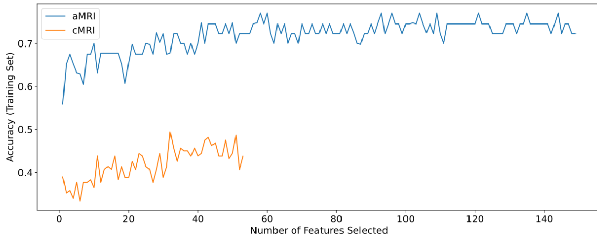
Figure 4. Model accuracy scores across the total feature set completed by recursive feature elimination in both the cMRI and aMRI groups. The cMRI group training accuracy began at ~39% accuracy compared to the aMRI group ~55% accuracy creating a 16% accuracy difference. Both models present an upward trend as more features are selected with the aMRI group beginning to plateau past 55 selected features. The cMRI group showed the greatest accuracy fluctuations around ~20-37 selected features with the aMRI group having the greatest accuracy fluctuations around ~0-25 selected features.
