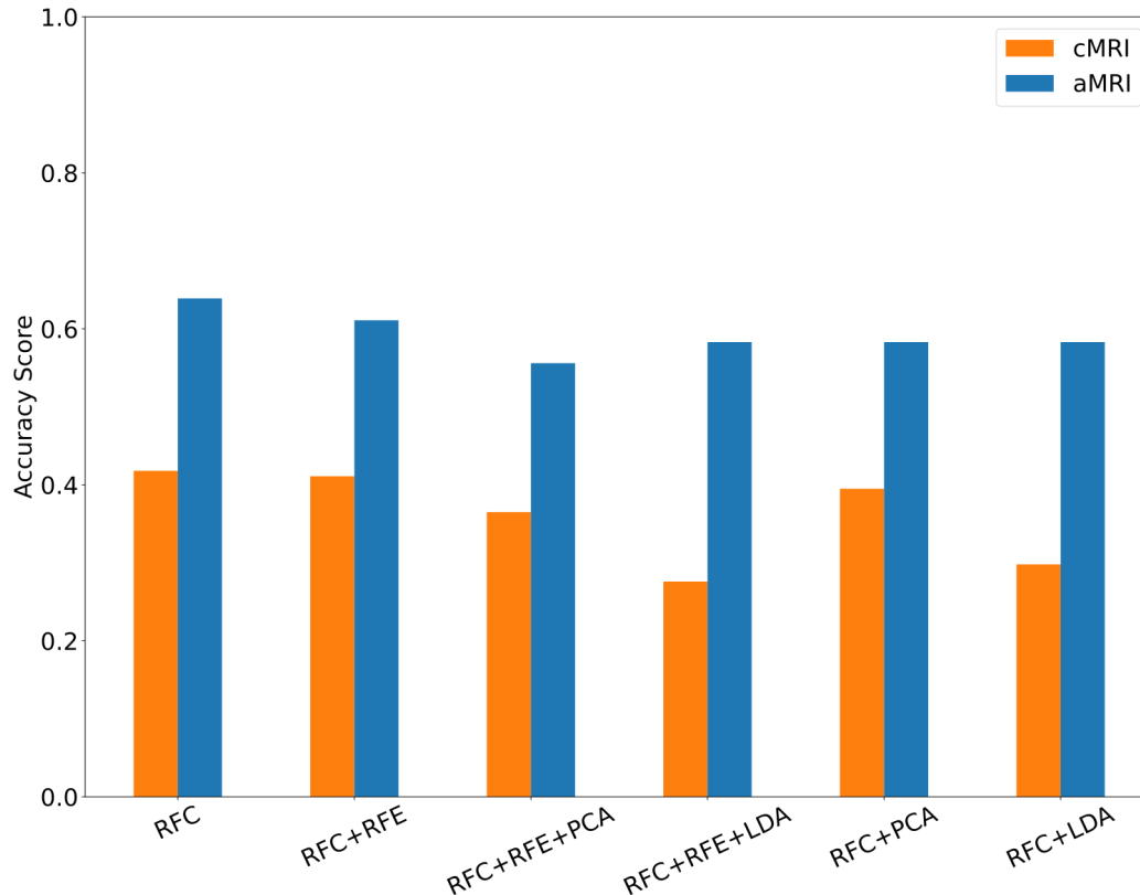
Figure 5. Accuracy score visualization for different model variations compared between the cMRI dataset and the aMRI dataset metrics. Both cMRI and aMRI dataset accuracies show minimal fluctuations between model variations. That being said, all the aMRI models outperform their cMRI counterparts. The largest difference between cMRI and aMRI accuracy scores is seen in the RFC+RFE+LDA model with a 30.7% prediction accuracy difference. The smallest difference between the cMRI and aMRI accuracy scores is seen in the RFC+PCA model with a 19.1% prediction accuracy difference.
