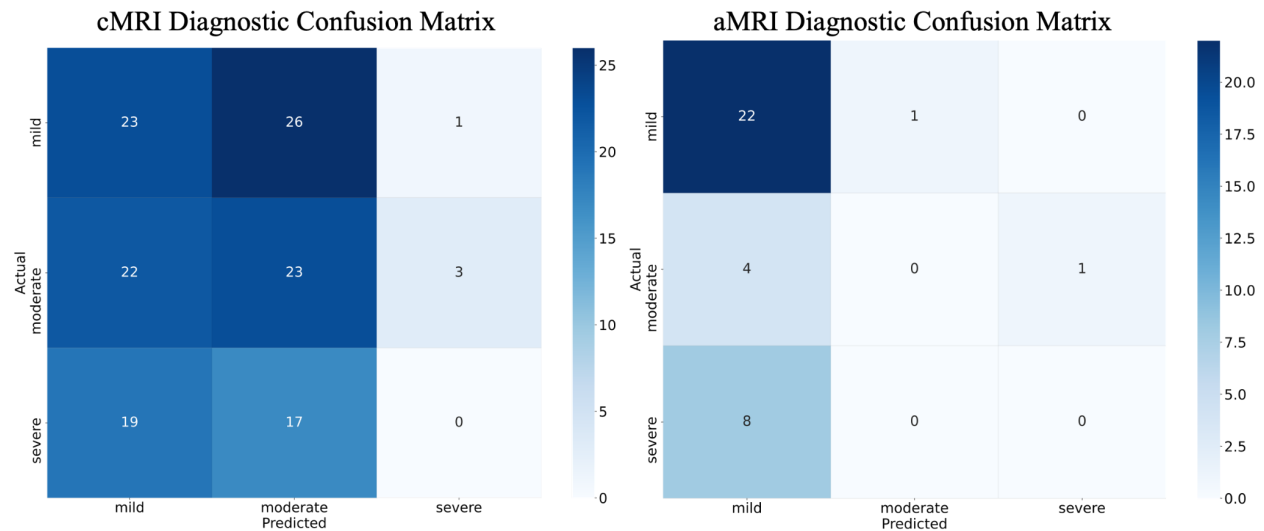
Figure 3. Confusion Matrix for cMRI and aMRI dataset model predictions across MJOA categories for baseline disease severity. The cMRI prediction model performed equally in predicting mild and moderate baseline disease severity with 23/50 correct and 23/48 correct respectively. The cMRI prediction model was not able to predict any of the 36 severe testing patients correctly. That being said, the model favours making moderate predictions (n=66) slightly more than mild predictions (n=64). It favours both mild and moderate predictions significantly more than severe predictions (n=4). The aMRI model predicts 22/23 mild patients correctly yet incorrectly the 5 moderate and 8 severe testing patients. It highly favours making mild predictions (n=34) as opposed to moderate or severe predictions (n=1 per group).
