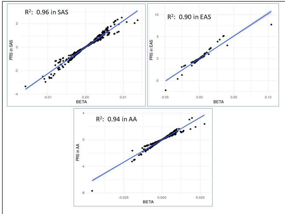
Figure 2: Pearson Correlation of PRS in SAS, EAS and AA showed the risk score obtained from all the 308 SNPs are showing strong correlation with the beta values (effective size)
