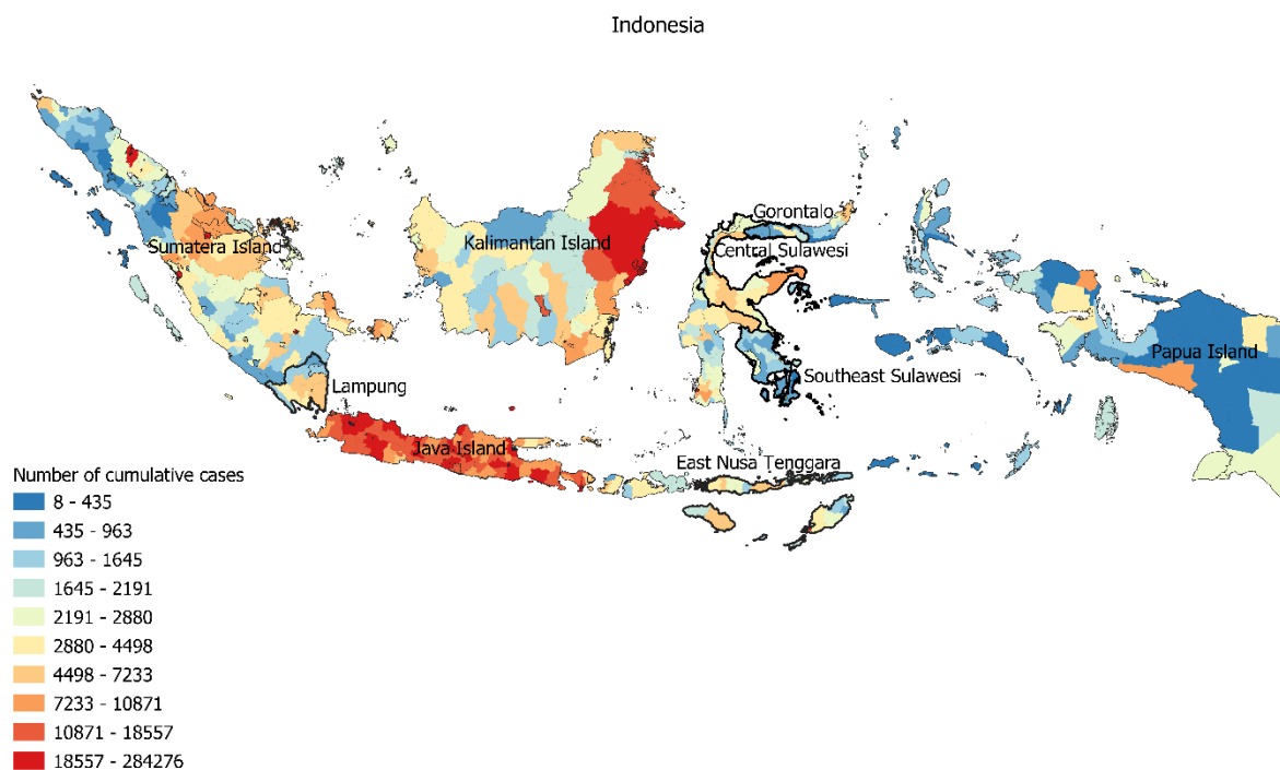
Figure 1: Map showing five study sites in Gorontalo, Lampung, East Nusa Tenggara, Central Sulawesi, and Southeast Sulawesi province, and spatial distribution of cumulative COVID-19 cases by district as per 27 February 2022. The administrative boundaries of the study sites were highlighted in bold. COVID-19 aggregated data were obtained from https://data.covid19.go.id/ .
