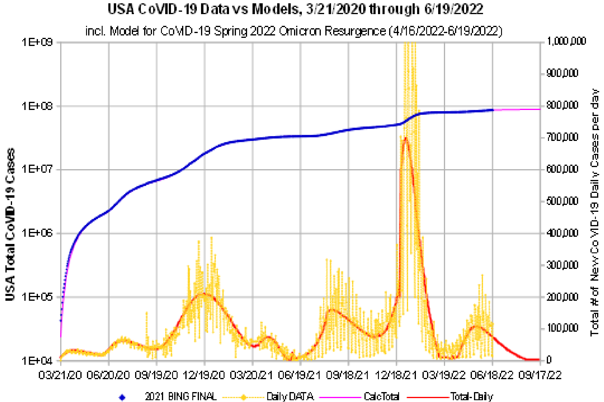
Fig. 4: USA CoVID-19 Daily and Total, w/ Spring 2022 Resurgence Data Fits: 3/21/2020- 6/19/2022
