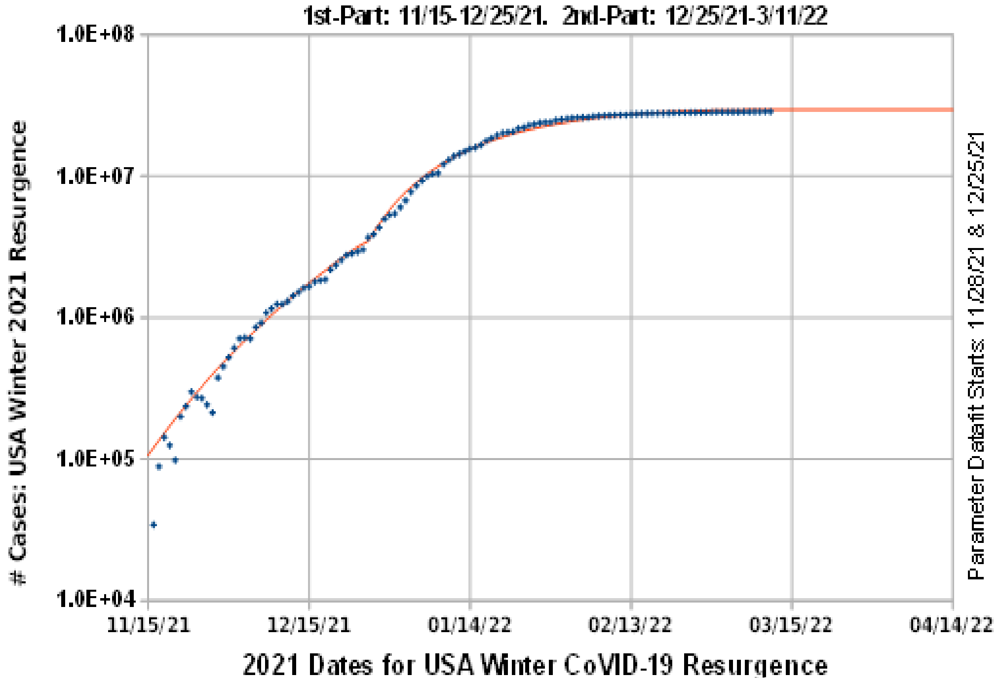
Fig. 1: Final USA Winter 2021 Omicron CoVID-19 Wave By Itself
