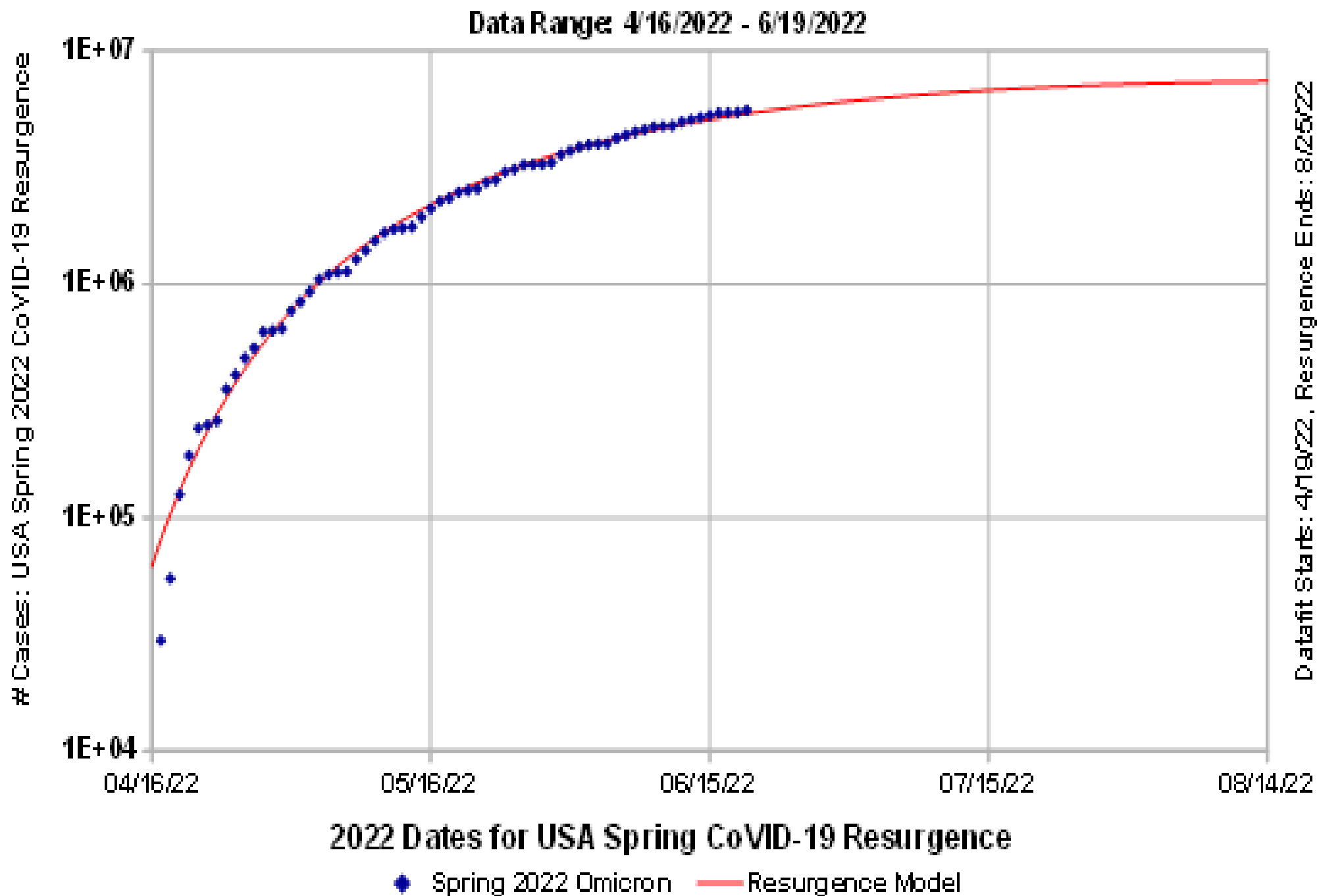
Fig. 3: USA CoVID-19 Spring 2022 Resurgence By Itself
