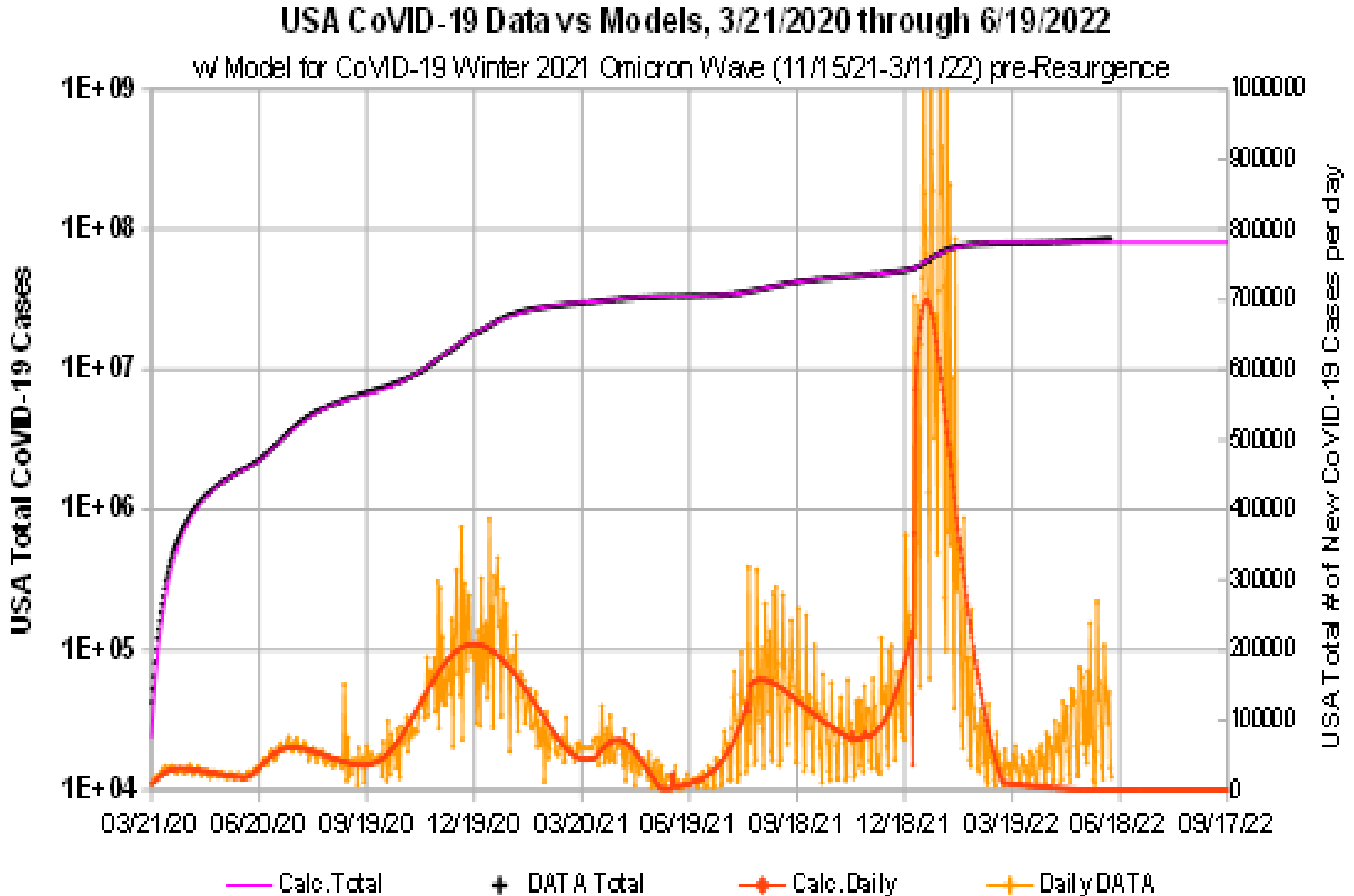
Fig. 2: USA CoVID-19 Totals w/ Data Fitting 3/21/2020 - 3/11/2022
