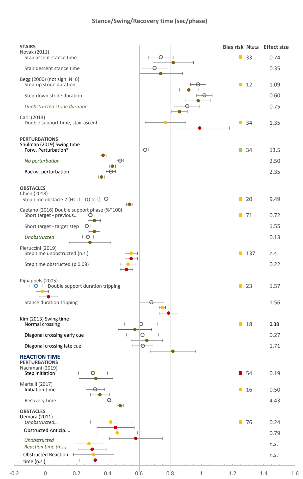
Figure 2: Forest plot of stance, swing or recovery time, below the reaction time. Circles: open blue— younger adults, yellow closed— older adults with low fall risk, red closed— older adults with high fall risk. (which was not certified by peer review) is the author/funder, who has granted medRxiv a license to display the preprint in perpetuity. Unspecified fall risk. CC-BY 4.0 International.
