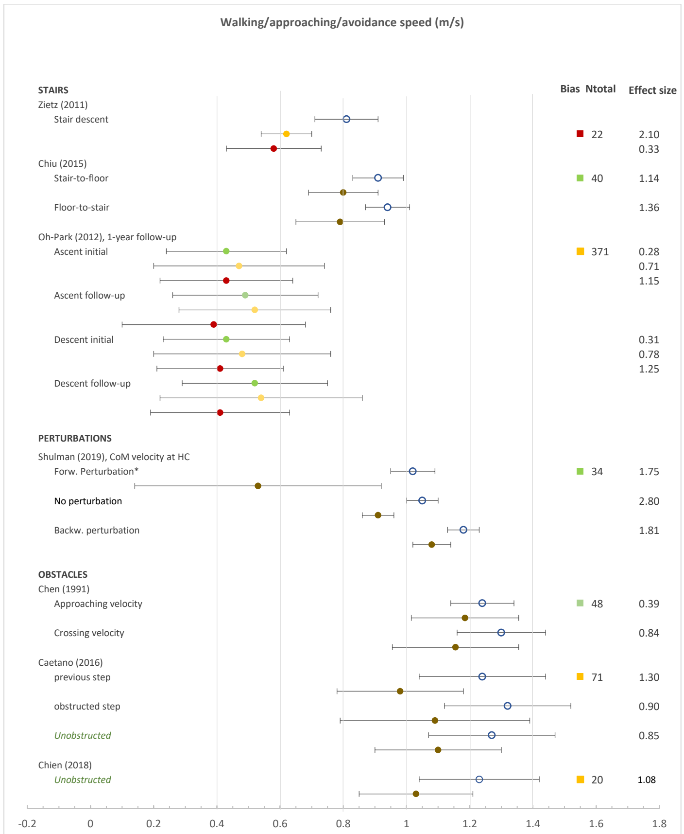
Figure 6: Forest plot of Velocity. Circles: open blue— younger adults, yellow closed— older adults with low fall risk, red closed— older adults with high fall risk, brown closed— older adults with unspecified fall risk. For Oh-Park (2012): older adults whose functional score improved/stayed the same / deteriorated after a year are indicated in green / yellow / red. CoM, centre of mass; HC, heel contact; min., minimum; ML, medial-lateral; MoS, margin of stability; n.s., not significant. Ntot is the total number of participants.
