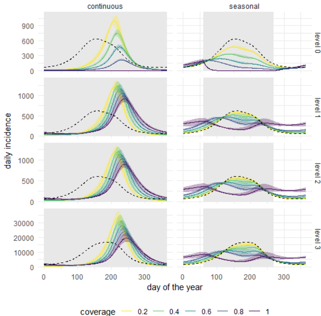
322 323 324 Fig. 2. Temporal changes in seasonal RSV incidence under different vaccination coverages and 325 strategies (seasonal vs. continuous, vaccination windows indicated by grey shaded areas) 326 compared to no vaccination (black dashed lines). Continuous vaccination leads to more narrow 327 epidemic peaks with larger amplitude and delayed peak timing at all levels for all coverages 328 (except 100% coverage at level 0). Seasonal vaccination at coverages less than 100% flattens 329 the epidemic peak at all levels. 100% seasonal coverage leads to two small peaks at the 330 beginning and the end of the regular season for levels 1-3.
