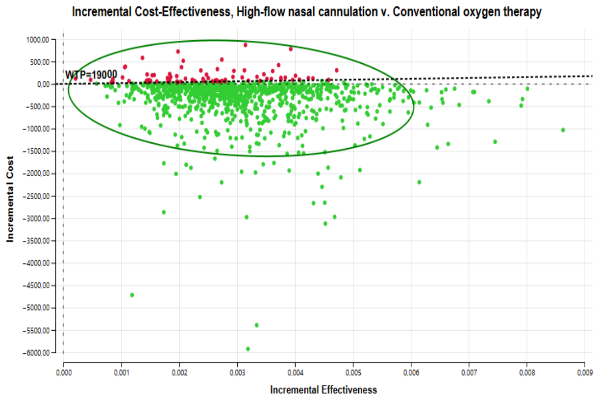
Figure 4. Cost effectiveness plane
