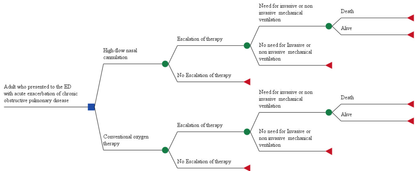
Figure 1. Decision tree model
