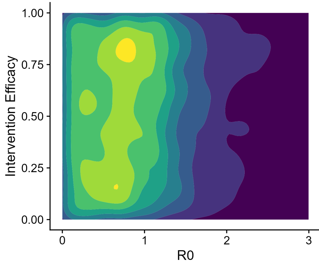
Figure 2: The posterior distribution of pairs of R_0 and intervention efficacy values, pooled across all MVD outbreaks. Lighter colours represent areas of higher density.
