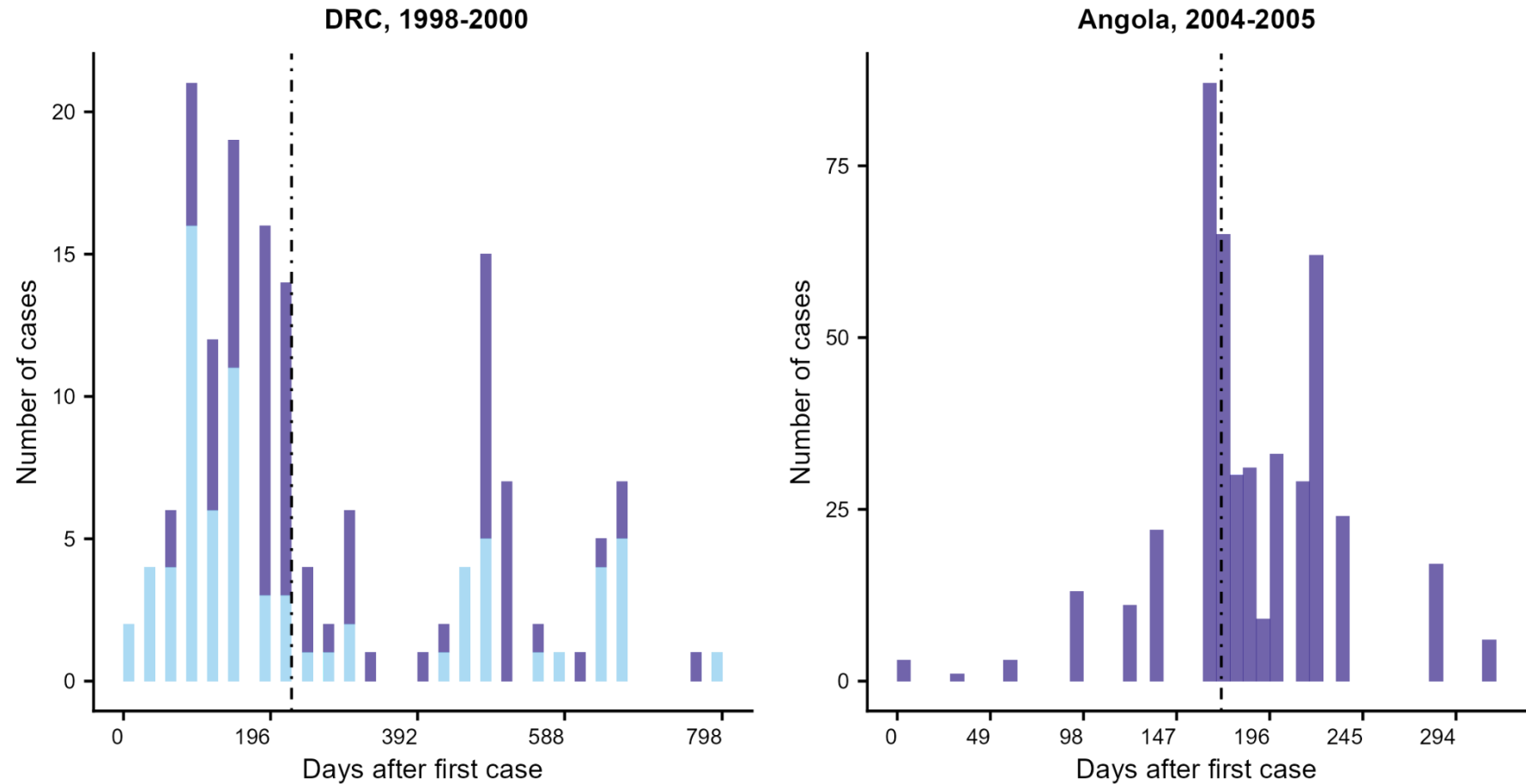
Figure 1: Incidence plots of Marburg virus disease outbreaks involving three or more confirmed or probable cases. Cases are plotted by onset date, except for the outbreak in Angola, which shows the day of reporting. Dashed lines represent the day on which interventions were put in place. Light blue bars indicate probable spillover infections to humans from animals and dark blue bars cases of human-to-human transmission.
