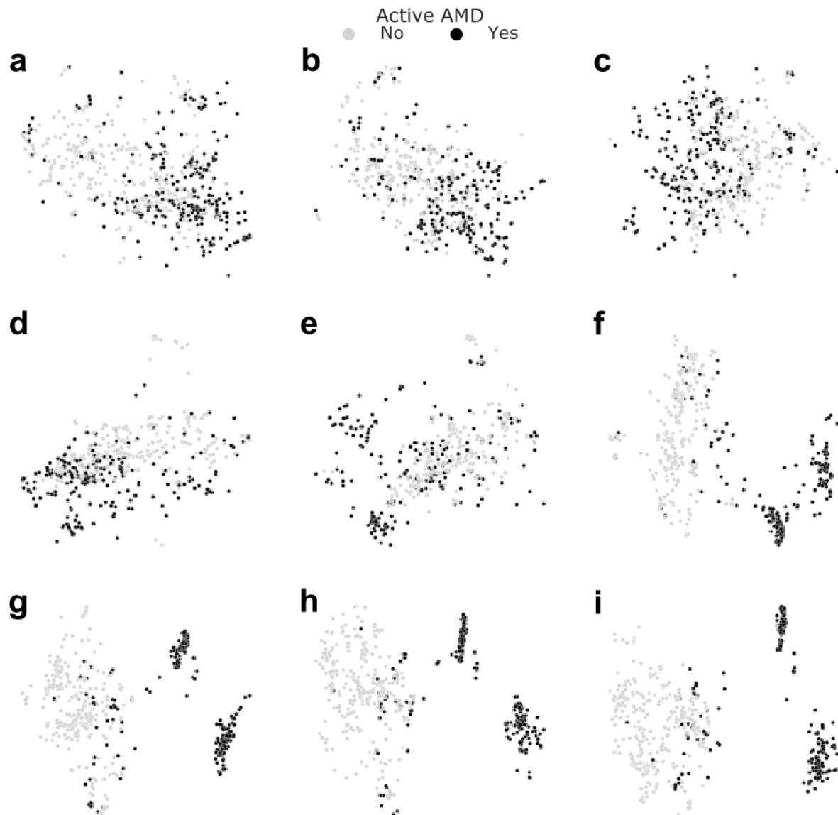
Figure 7: Layer-wise visualization of test data via t-SNE. Starting just before the first Inception module (a) and reading out feature representations yielded by every other module (b-f) along with the last Inception module (g), the shared representation layer (h) and the nAMD activity detection head's penultimate layer (i), we performed t-SNE with the aforementioned settings. Useful representations emerged towards the end of convolutional stack and the task-specific representation allowed the best separation of nAMD active cases from those inactive. Exact read-out locations can be found in Fig. 8.
