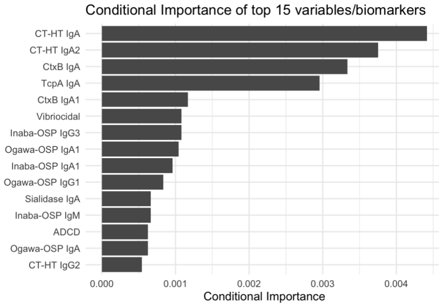
211 Figure 5. Biomarkers important for classifying vaccinees by whether they developed diarrhea 212 following V. cholerae challenge. Top 15 biomarkers important in classifying vaccinees by developing 213 either no qualifying diarrhea or mild to severe diarrhea following V. cholerae challenge. Biomarkers were 214 selected using serum collected from participants on the day of challenge. Biomarkers are ranked by 215 importance scores calculated using conditional random forest classification models. 216
