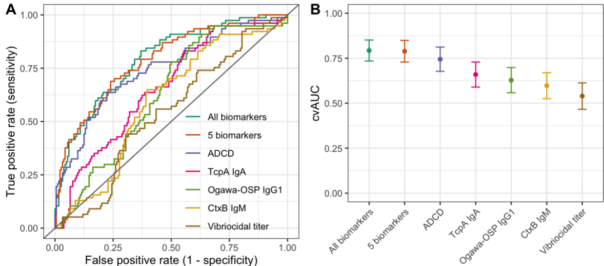
171 172 Figure 4. Predicting infection outcome among household contacts using different subsets of 173 biomarkers. A) Cross-validated receiver operator curves (cvROC) for classifying household contacts of 174 index cholera cases that remain uninfected vs. become infected using random forest models with different 175 subsets of biomarkers and age. “5 biomarkers” corresponds to five of the top biomarkers selected via 176 conditional importance, including ADCD, CtxB IgM, TcpA IgG2, Ogawa-OSP IgG1, and Sialidase IgG1. 177 True and false positive rates calculated using leave-one-out cross-validation. B) Cross-validated area 178 under the curve (cvAUC) corresponding to the models in A. Influence-curve based 95% confidence 179 intervals are shown for the cvAUC estimates.
