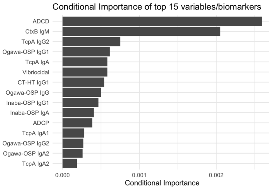
155 156 Figure 3. Biomarkers important for classifying household contacts by infection outcome. Top 15 157 biomarkers important in classifying household contacts of index cholera cases as infected (i.e., becoming 158 stool culture positive) vs. uninfected (i.e., remaining stool culture negative). Biomarkers are ranked by 159 importance scores calculated using conditional random forest classification models. 160
