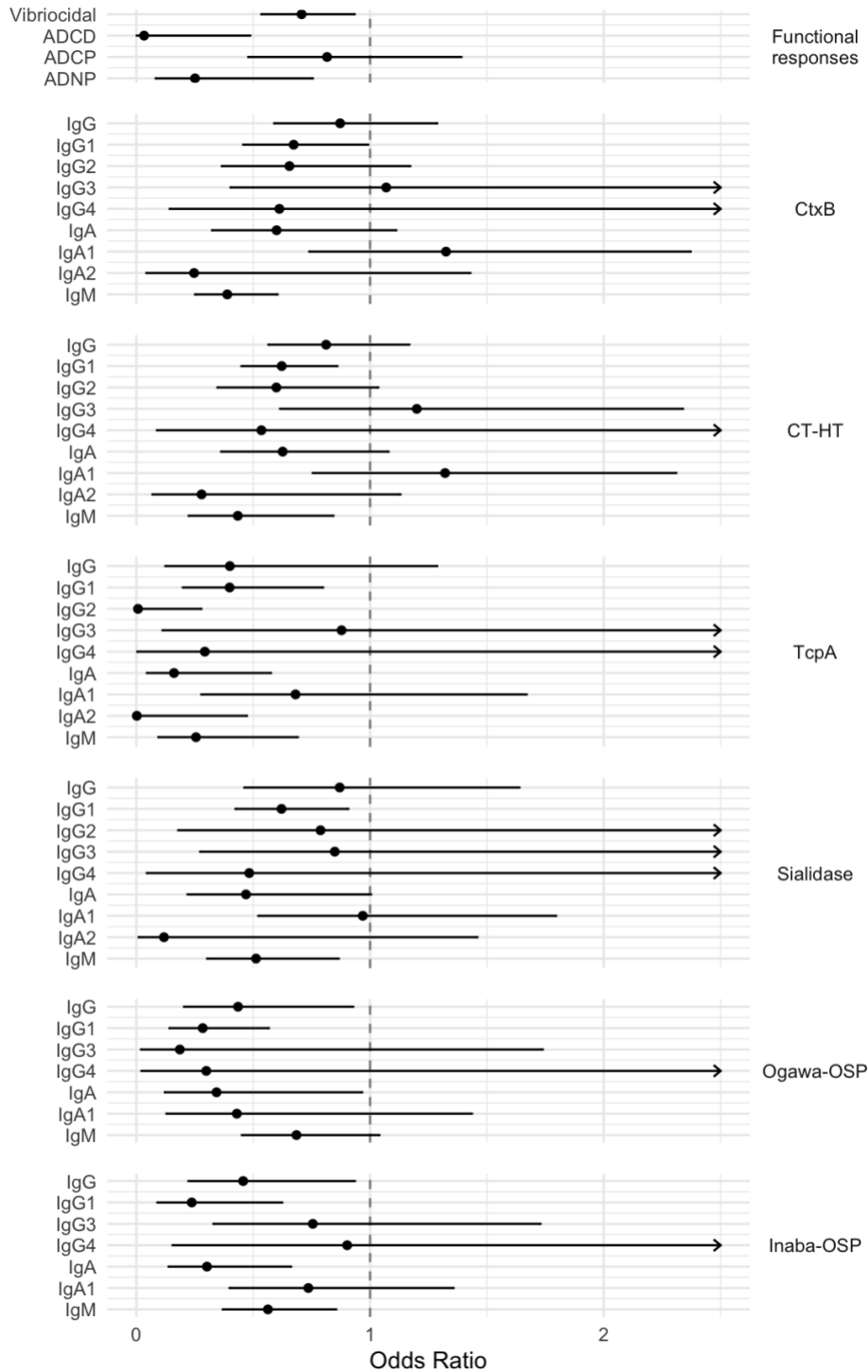
143 Figure 2. Risk of infection in household contacts of an index cholera case. Odds ratio of becoming 144 infected among household contacts of an index cholera case for every 2-fold increase in baseline (Day 2) 145 antibody titers, after adjusting for age and household clustering. Mean and 95% confidence interval are 146 shown for each biomarker analyzed independently. Arrows indicate where upper confidence interval 147 extends beyond the graph. Isotype is indicated on the left and antigen on the right for binding antibody 148 titers. Biomarkers for which logistic model fitted values were very close to 1 are excluded.
