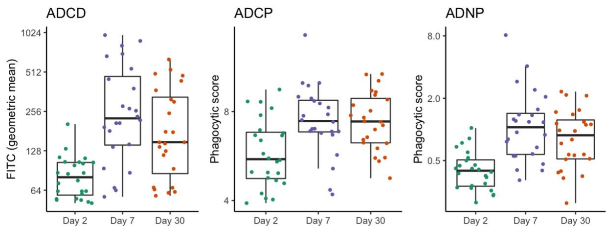
125 Figure 1. Dynamics of functional antibody responses targeting the V. cholerae O1 antigen 126 following V. cholerae infection. Antibody-dependent complement deposition (ADCD), cellular 127 phagocytosis (ADCP), and neutrophil phagocytosis (ADNP) in serum from 24 index cholera cases upon 128 enrollment (i.e., Day 2 post presumed symptom onset) and days 7 and 30 post onset. Each point 129 represents the geometric mean of complement deposition and phagocytic scores, respectively, across 130 three replicates. Boxplots show 50% (median), 25%, and 75% quartiles; whiskers represent approximate 131 95% confidence intervals for comparing medians (McGill et al., 1978).
