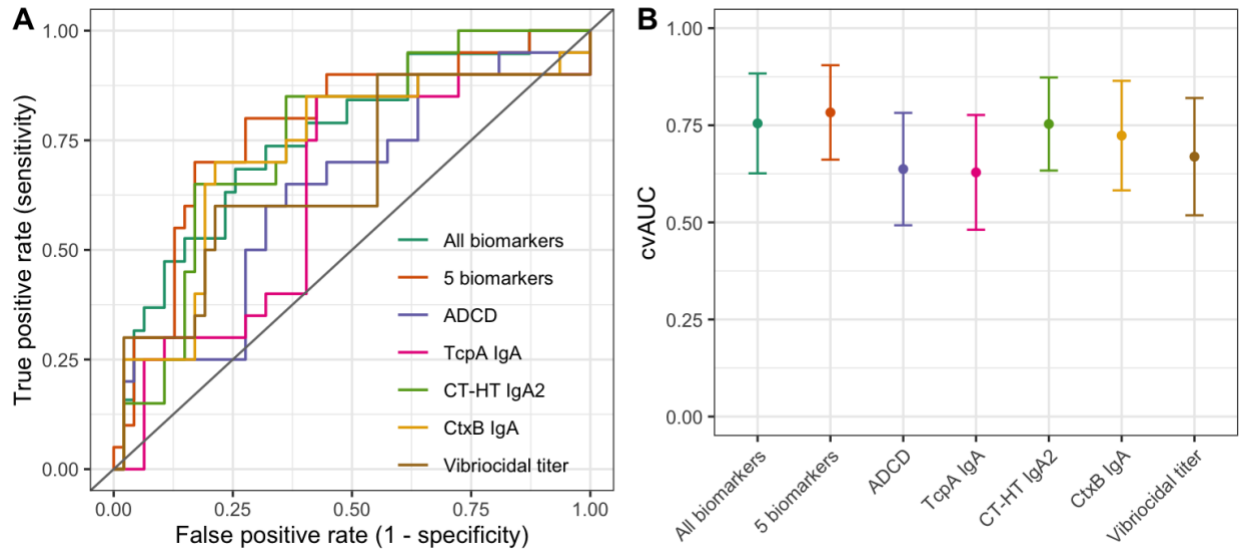
230 Figure 6. Predicting whether vaccinees develop diarrhea using different subsets of biomarkers. A)
