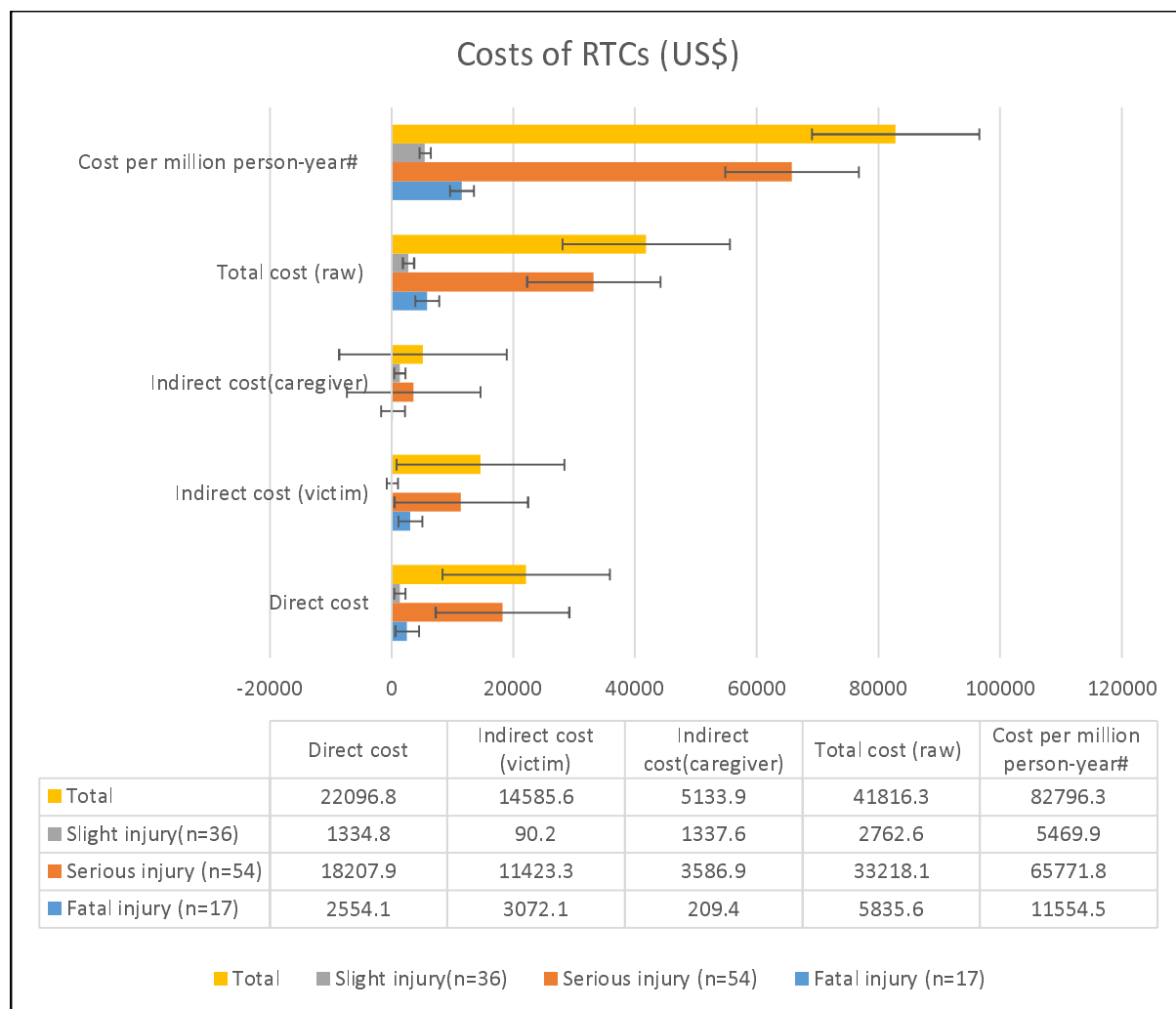
Fig. 2. Costs of RTCs in US $ (US $1 =NRs 102.92 as per 2017, Jun 1) with standard error bars;
