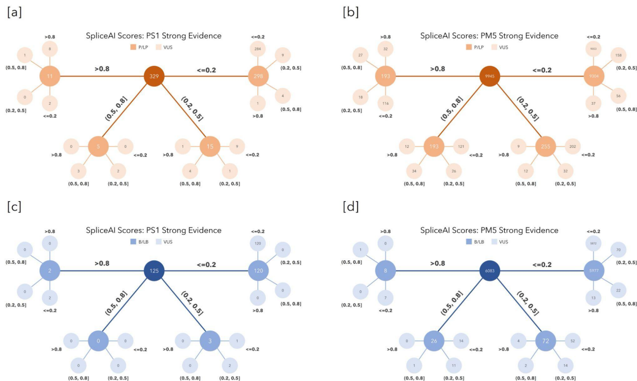
Figure 3: SpliceAI scores of related variants. To evaluate how frequently variants with discordant classifications may be attributable to different splicing impacts, we use SpliceAI. Score ranges of >0.8 , >0.5 and \leq 0.8 , >0.2 and \leq 0.5 , and \leq 0.2 represent high, intermediate, weak, and low predicted impacts on splicing, respectively. [a] SpliceAI scores for P/LP-VUS PS1 variant pairs. In 86.3% of pairs ( N=284 ), both variants have low predicted splicing impact. [b] SpliceAI scores for P/LP-VUS PM5 variant pairs. In 91.0% of pairs ( N=9,053 ), both variants have scores \leq 0.2 . [c] SpliceAI scores for B/LB-VUS PS1 variant pairs. In 96.0% of pairs ( N=120 ), both variants have scores \leq 0.2 . [d] SpliceAI scores for B/LB-VUS PM5 variant pairs. In 96.5% of pairs ( N=5,872 ), both variants have scores \leq 0.2 .
