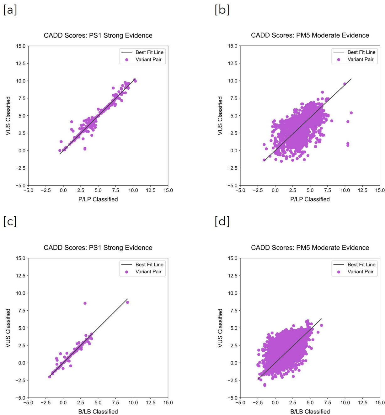
Figure 2: CADD scores of variant pairs are correlated. Individual points represent variant pairs where one variant has a known annotation (P/LP or B/LB) and there is a related VUS affecting the same codon. Each dot compares the CADD score of the variant with an annotation to that of the related VUS. [a] CADD scores for P/LP-VUS PS1 variant pairs. The variant pairs
