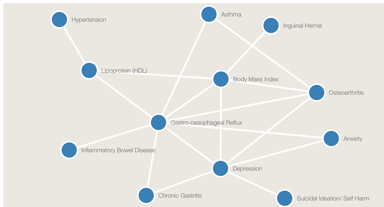
Figure 2: Genetic disease network of depression. For all connections observed in the phenotypic network of depression (figure 1), we evaluated the pairwise genetic correlation using LDSC(14). Edges in the graph show all significant genetic correlations between traits after correcting for multiple hypothesis testing.
