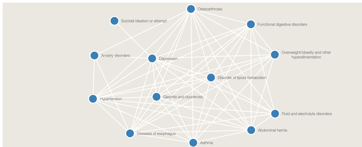
Figure 1: Phenotypic disease network of depression. The disease network of depression was obtained from the fully connected phenotypic network using phenotypic correlations as edge weights, by reducing the dense graph to a sparse network by keeping only the top 1% of the connections and extracting depression and its immediate neighbour nodes.
