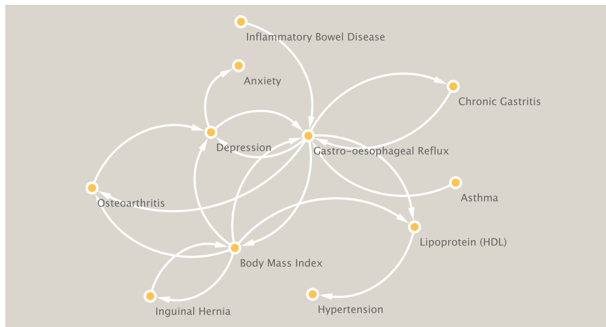
Figure 3: Causal relationships between traits that are comorbid with depression. We tested causal relationships between traits and depression using bidirectional Mendelian randomization for all genetically correlated pairs of disorders. Using SNP effects as instrumental variables, the resulting directed graph shows significant causalities between traits after correcting for multiple hypothesis testing.
