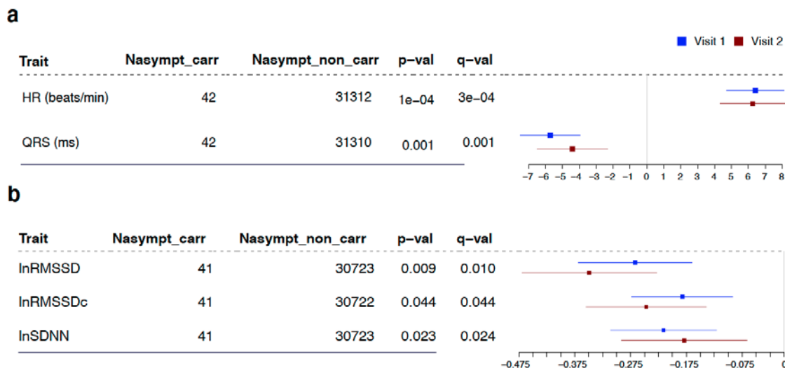
Figure 2. Forest plot of effect sizes for significant quantitative phenotypes. Squares represent the effect size (beta). Lines represent standard error. Blue shapes and the numbers in the columns correspond to analysis results for the baseline visit (visit 1). Red shapes correspond to the second visit approximately 5-years later (visit 2). Phenotypes are separated by the scale in a) and b) panels. Nasympt_carr , number of asymptomatic carriers with non-null information in visit 1; Nasympt_non_carr , numbers of asymptomatic non-carriers with non-null information in visit 1; p-val : p-value for the independent association; q-val : false discovery rate for conjoined analysis of all the traits that takes into account 100 permutations for each of the 38 traits; lnRMSSD : natural logarithm of the root mean square of successive differences; lnRMSSDc : RMSSD corrected by heart rate; lnSDNN : natural logarithm of the normal-to-normal intervals.
