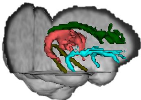
Figure 1. Key fronto-limbic white matter tracts in a representative healthy, term-born neonate. Tracts of interest include the dorsal (green) and inferior (gold) cingulum bundle, fornix (pink), and uncinate (blue).
