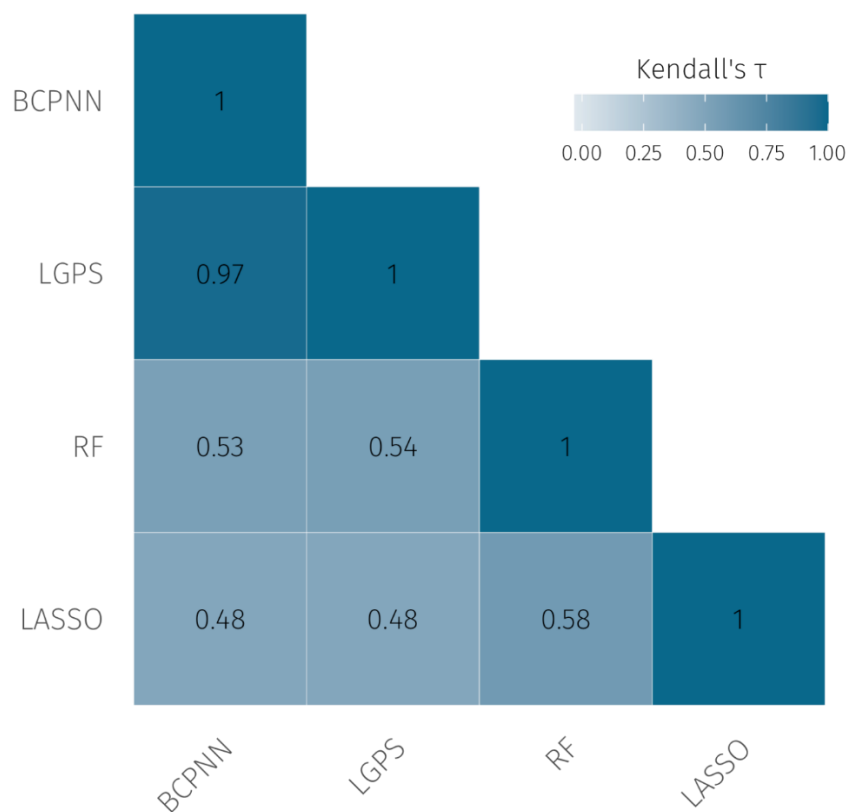
Figure 2: Kendall's tau correlations between the rankings of the BCPNN, LGPS, RF and LASSO. The disproportionality methods, BCPNN and LGPS, lead to similar rankings. The LASSO and the RF, however, differ substantially from the others. We reduced the range of the legend for readability.
